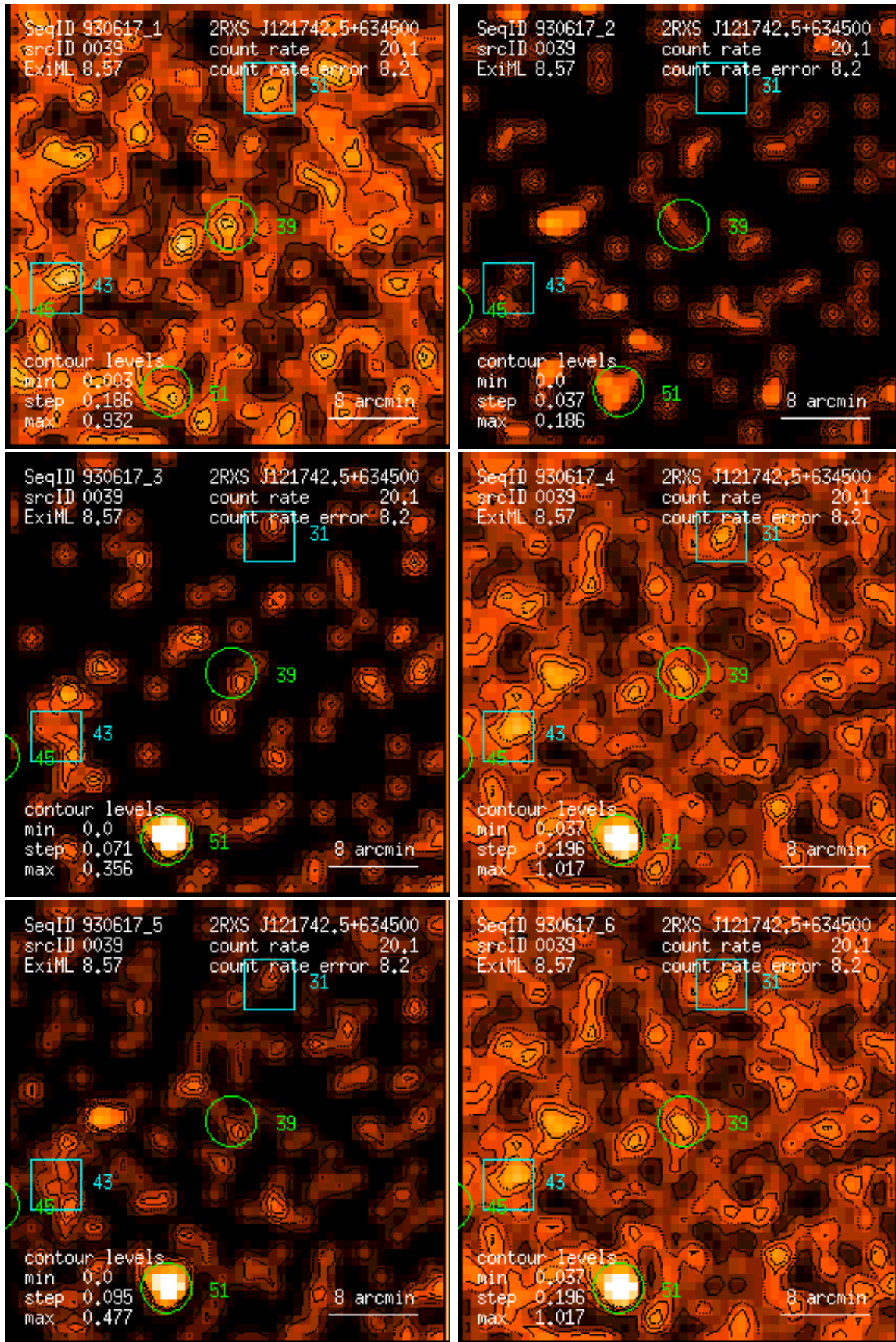
Figure 39: RASS 930617: detection 0039: band rate images, Gaussian filter: (1) PSPC channels 11 – 41, (2) 52 – 90, (3) 91 – 201, (4) 11 – 235, (5) 52 – 201, (6) 11 – 201. Broad band rates in counts/ks. Band rate contour levels in counts/ks/arcmin 2 .
