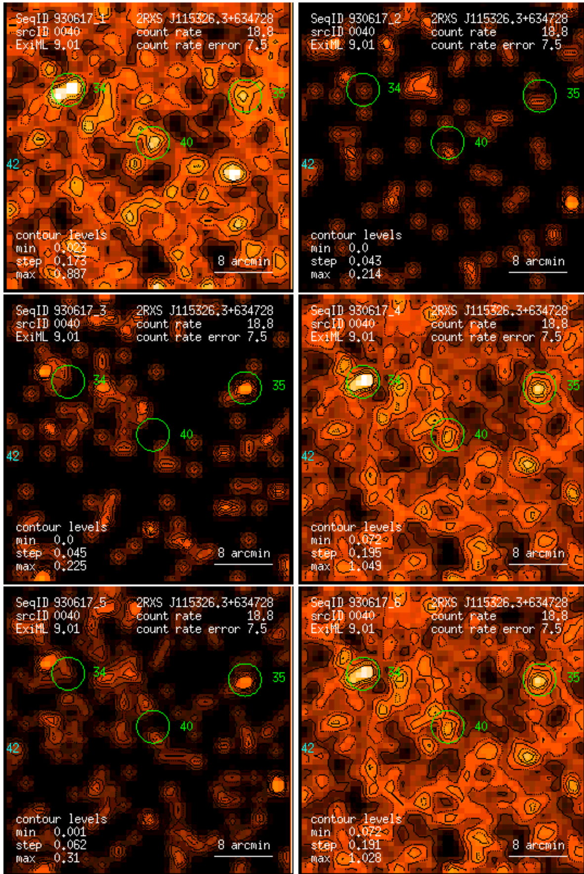
Figure 40: RASS 930617: detection 0040: band rate images, Gaussian filter: (1) PSPC channels 11 – 41, (2) 52 – 90, (3) 91 – 201, (4) 11 – 235, (5) 52 – 201, (6) 11 – 201. Broad band rates in counts/ks. Band rate contour levels in counts/ks/arcmin 2 .
