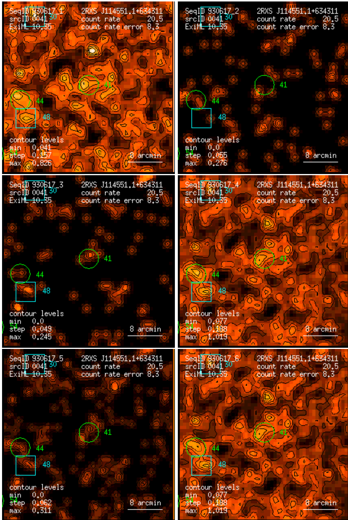
Figure 41: RASS 930617: detection 0041: band rate images, Gaussian filter: (1) PSPC channels 11 – 41, (2) 52 – 90, (3) 91 – 201, (4) 11 – 235, (5) 52 – 201, (6) 11 – 201. Broad band rates in counts/ks. Band rate contour levels in counts/ks/arcmin 2 .
