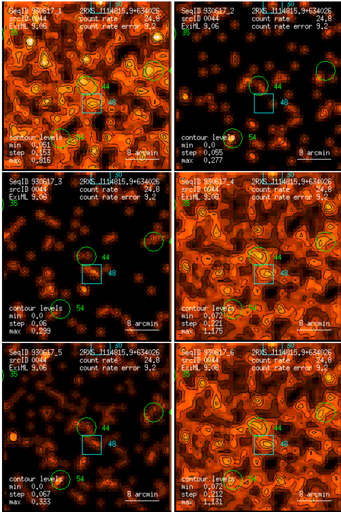
Figure 44: RASS 930617: detection 0044: band rate images, Gaussian filter: (1) PSPC channels 11 – 41, (2) 52 – 90, (3) 91 – 201, (4) 11 – 235, (5) 52 – 201, (6) 11 – 201. Broad band rates in counts/ks. Band rate contour levels in counts/ks/arcmin 2 .
