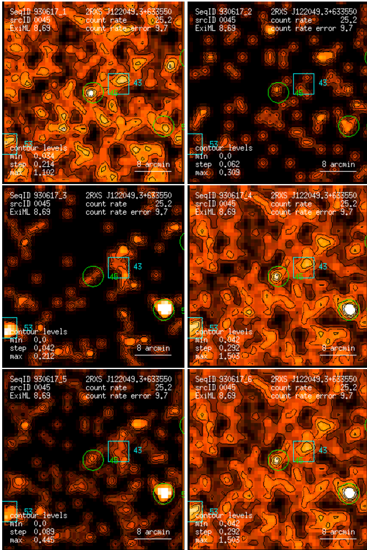
Figure 45: RASS 930617: detection 0045: band rate images, Gaussian filter: (1) PSPC channels 11 – 41, (2) 52 – 90, (3) 91 – 201, (4) 11 – 235, (5) 52 – 201, (6) 11 – 201. Broad band rates in counts/ks. Band rate contour levels in counts/ks/arcmin 2 .
