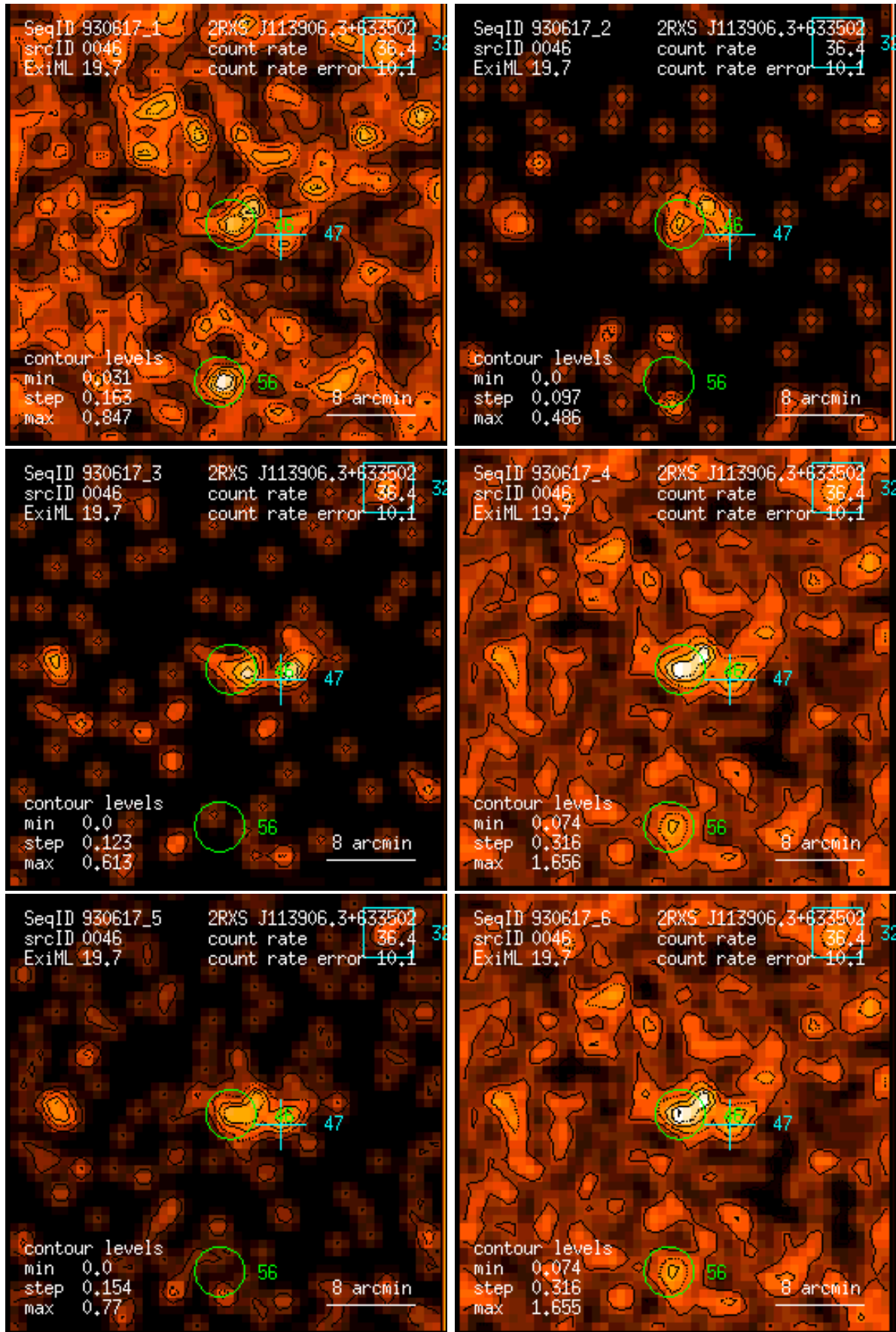
Figure 46: RASS 930617: detection 0046: band rate images, Gaussian filter: (1) PSPC channels 11 – 41, (2) 52 – 90, (3) 91 – 201, (4) 11 – 235, (5) 52 – 201, (6) 11 – 201. Broad band rates in counts/ks. Band rate contour levels in counts/ks/arcmin 2 .
