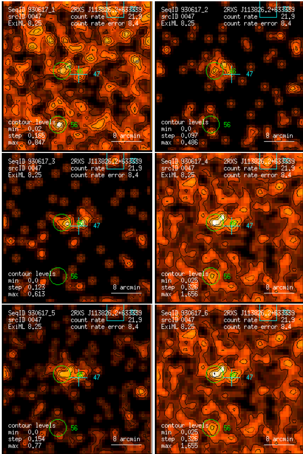
Figure 47: RASS 930617: detection 0047: band rate images, Gaussian filter: (1) PSPC channels 11 – 41, (2) 52 – 90, (3) 91 – 201, (4) 11 – 235, (5) 52 – 201, (6) 11 – 201. Broad band rates in counts/ks. Band rate contour levels in counts/ks/arcmin 2 .
