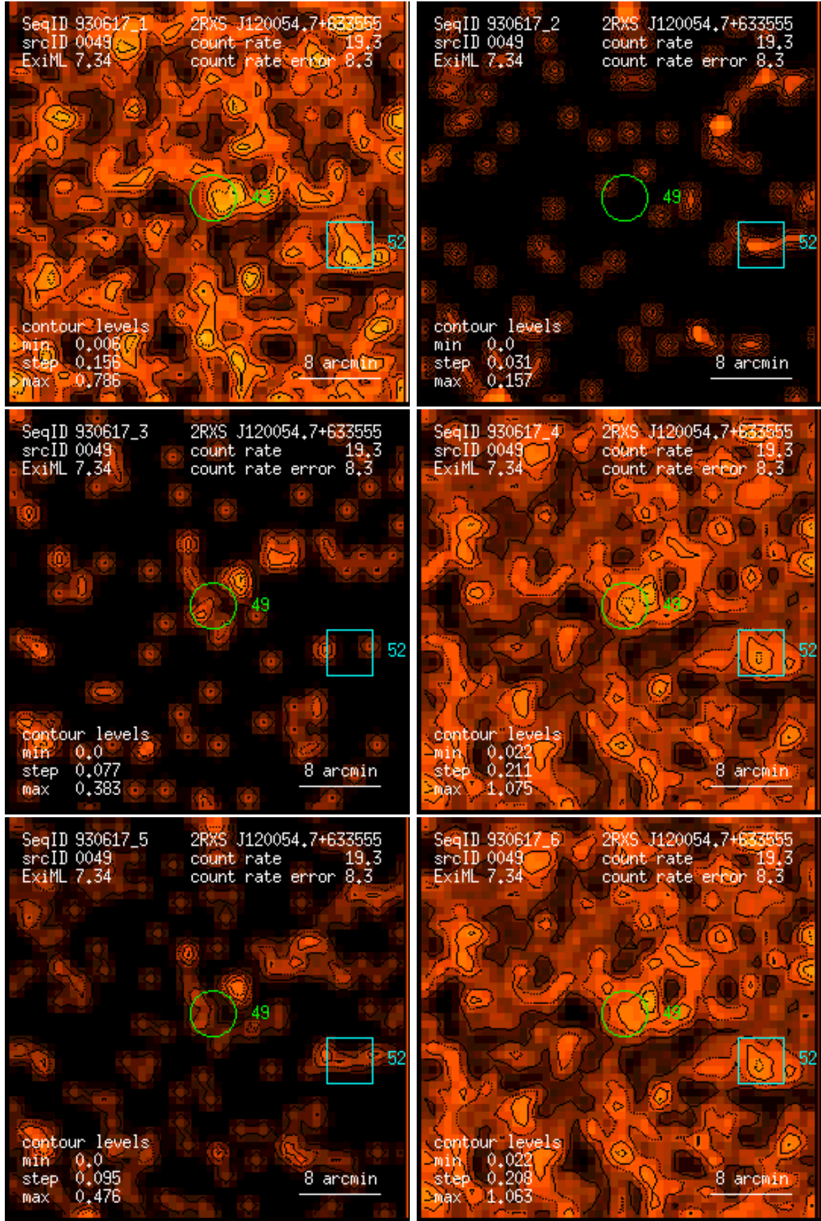
Figure 49: RASS 930617: detection 0049: band rate images, Gaussian filter: (1) PSPC channels 11 – 41, (2) 52 – 90, (3) 91 – 201, (4) 11 – 235, (5) 52 – 201, (6) 11 – 201. Broad band rates in counts/ks. Band rate contour levels in counts/ks/arcmin 2 .
