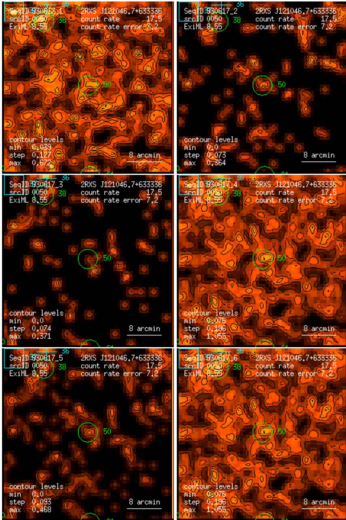
Figure 50: RASS 930617: detection 0050: band rate images, Gaussian filter: (1) PSPC channels 11 – 41, (2) 52 – 90, (3) 91 – 201, (4) 11 – 235, (5) 52 – 201, (6) 11 – 201. Broad band rates in counts/ks. Band rate contour levels in counts/ks/arcmin 2 .
