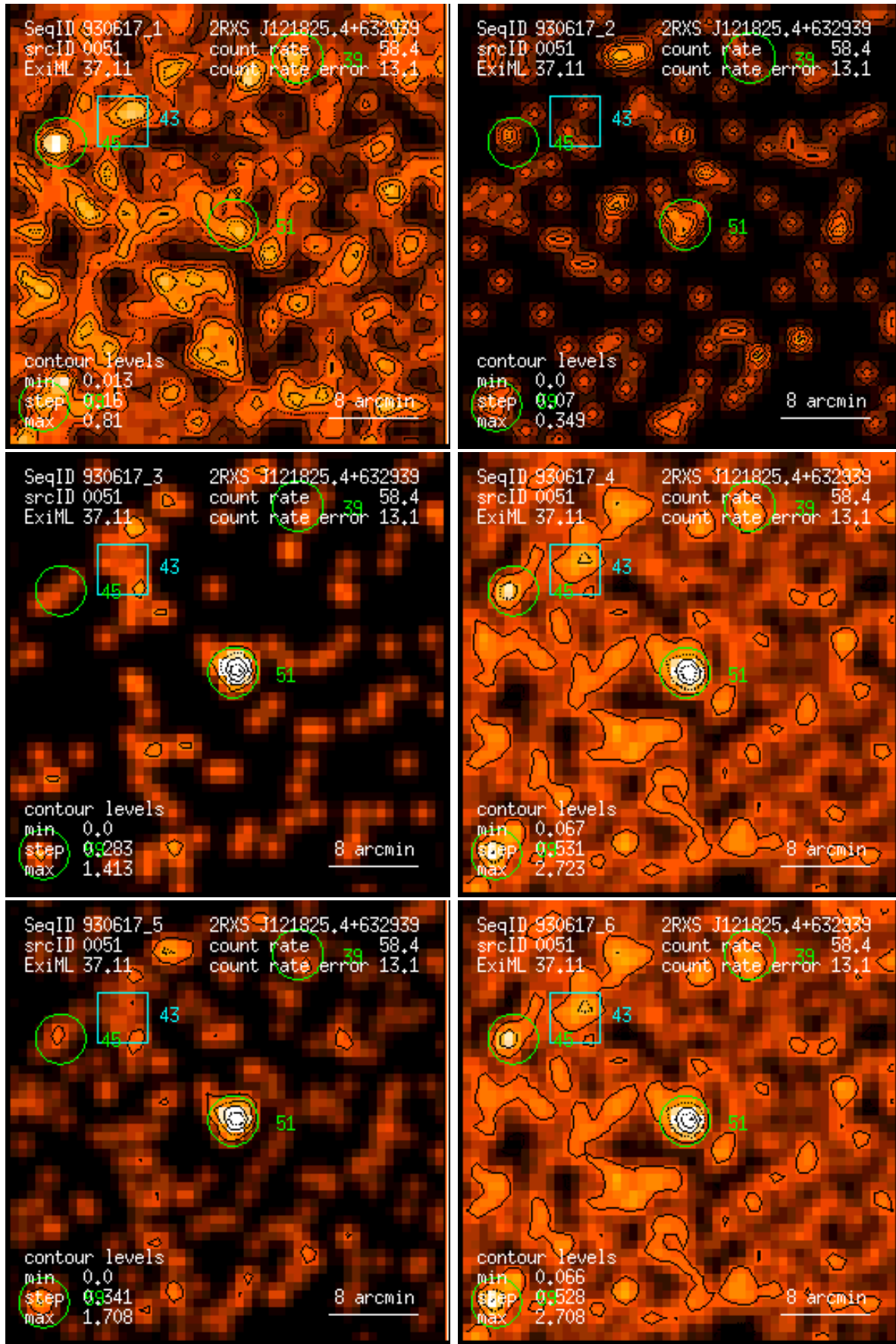
Figure 51: RASS 930617: detection 0051: band rate images, Gaussian filter: (1) PSPC channels 11 – 41, (2) 52 – 90, (3) 91 – 201, (4) 11 – 235, (5) 52 – 201, (6) 11 – 201. Broad band rates in counts/ks. Band rate contour levels in counts/ks/arcmin 2 .
