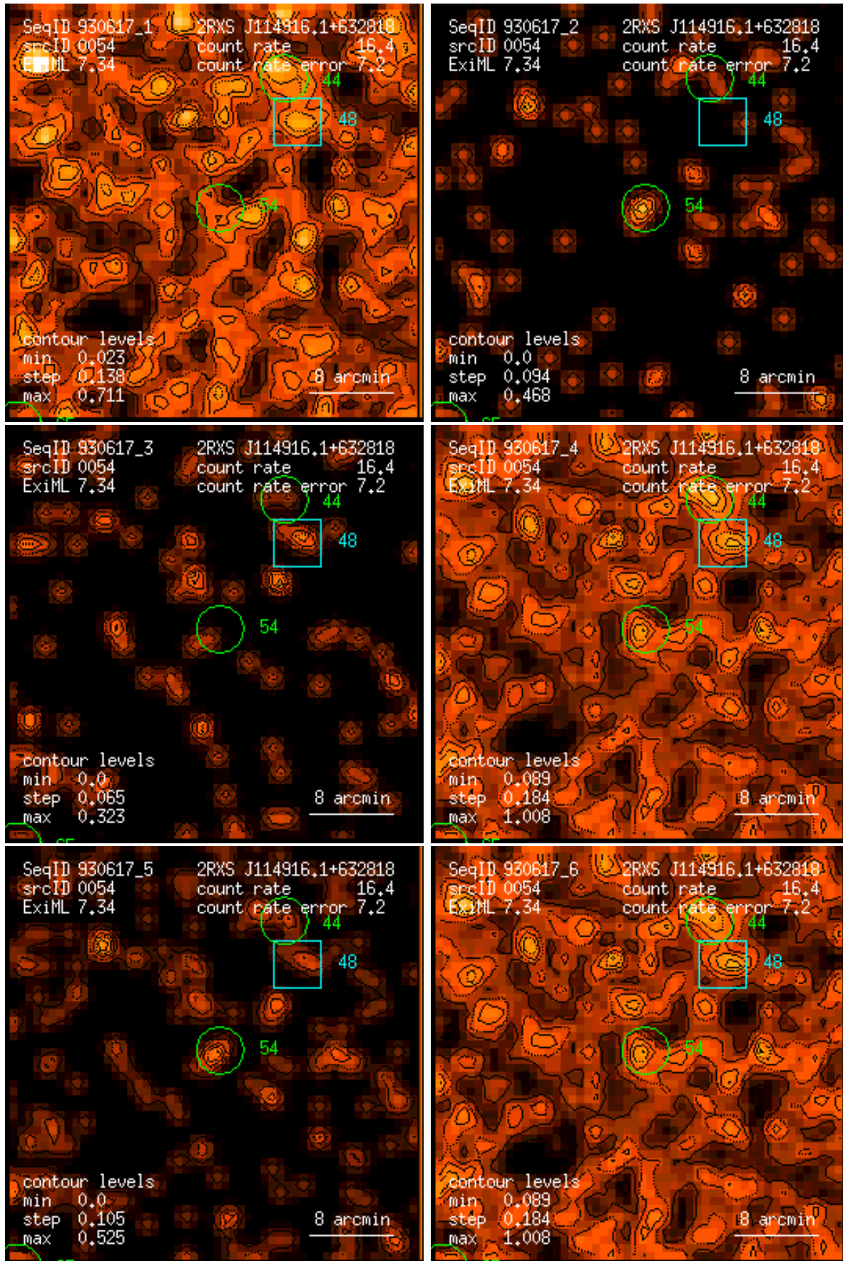
Figure 54: RASS 930617: detection 0054: band rate images, Gaussian filter: (1) PSPC channels 11 – 41, (2) 52 – 90, (3) 91 – 201, (4) 11 – 235, (5) 52 – 201, (6) 11 – 201. Broad band rates in counts/ks. Band rate contour levels in counts/ks/arcmin 2 .
