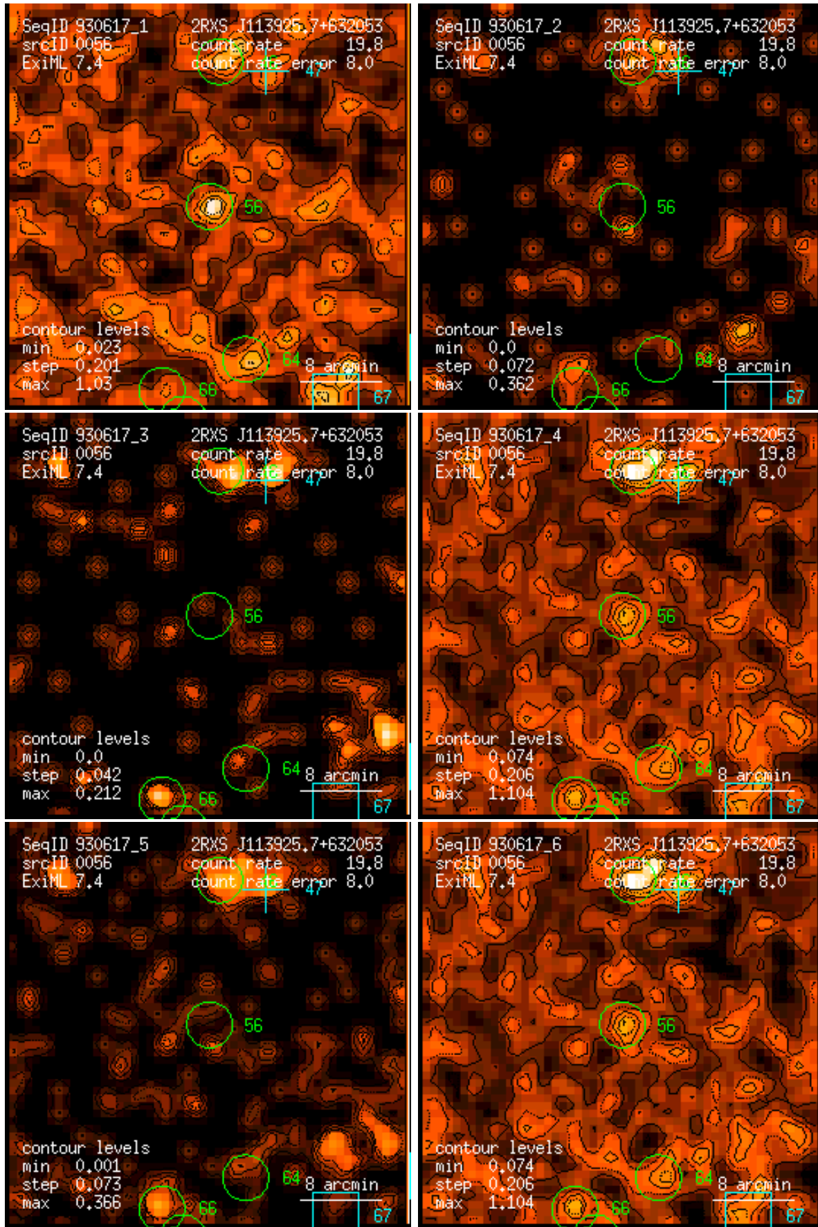
Figure 56: RASS 930617: detection 0056: band rate images, Gaussian filter: (1) PSPC channels 11 – 41, (2) 52 – 90, (3) 91 – 201, (4) 11 – 235, (5) 52 – 201, (6) 11 – 201. Broad band rates in counts/ks. Band rate contour levels in counts/ks/arcmin 2 .
