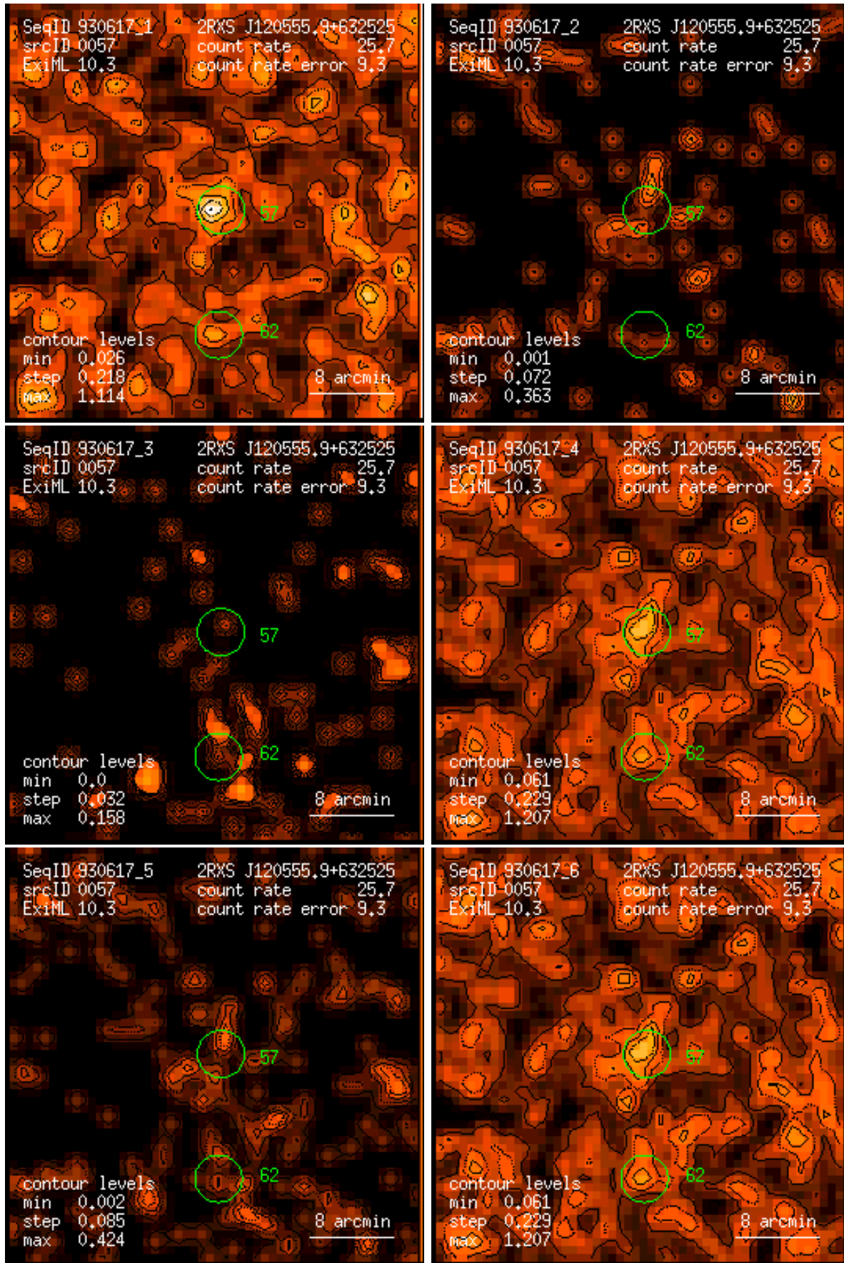
Figure 57: RASS 930617: detection 0057: band rate images, Gaussian filter: (1) PSPC channels 11 – 41, (2) 52 – 90, (3) 91 – 201, (4) 11 – 235, (5) 52 – 201, (6) 11 – 201. Broad band rates in counts/ks. Band rate contour levels in counts/ks/arcmin 2 .
