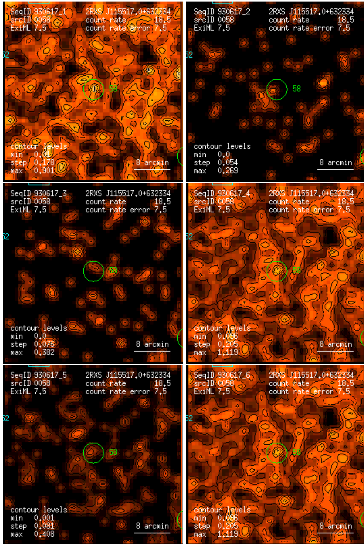
Figure 58: RASS 930617: detection 0058: band rate images, Gaussian filter: (1) PSPC channels 11 – 41, (2) 52 – 90, (3) 91 – 201, (4) 11 – 235, (5) 52 – 201, (6) 11 – 201. Broad band rates in counts/ks. Band rate contour levels in counts/ks/arcmin 2 .
