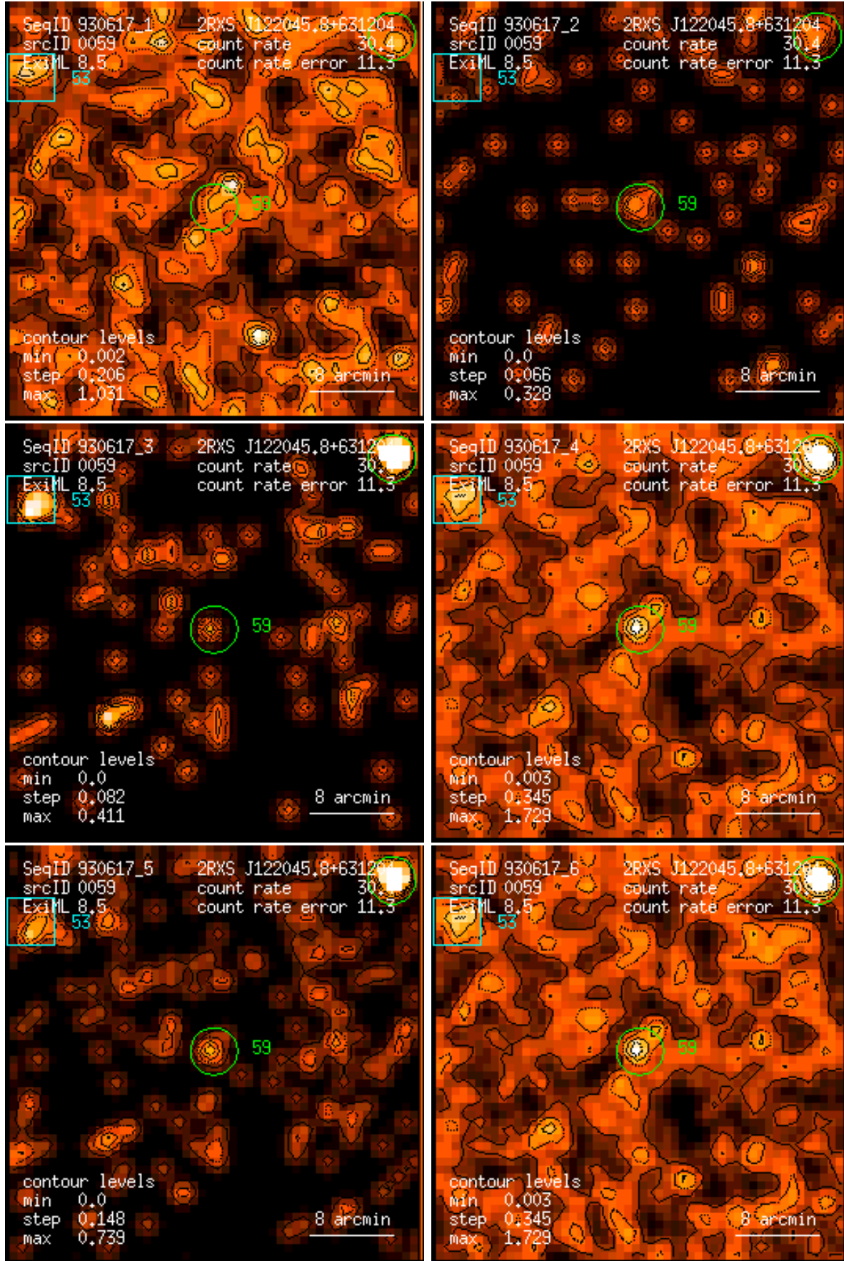
Figure 59: RASS 930617: detection 0059: band rate images, Gaussian filter: (1) PSPC channels 11 – 41, (2) 52 – 90, (3) 91 – 201, (4) 11 – 235, (5) 52 – 201, (6) 11 – 201. Broad band rates in counts/ks. Band rate contour levels in counts/ks/arcmin 2 .
