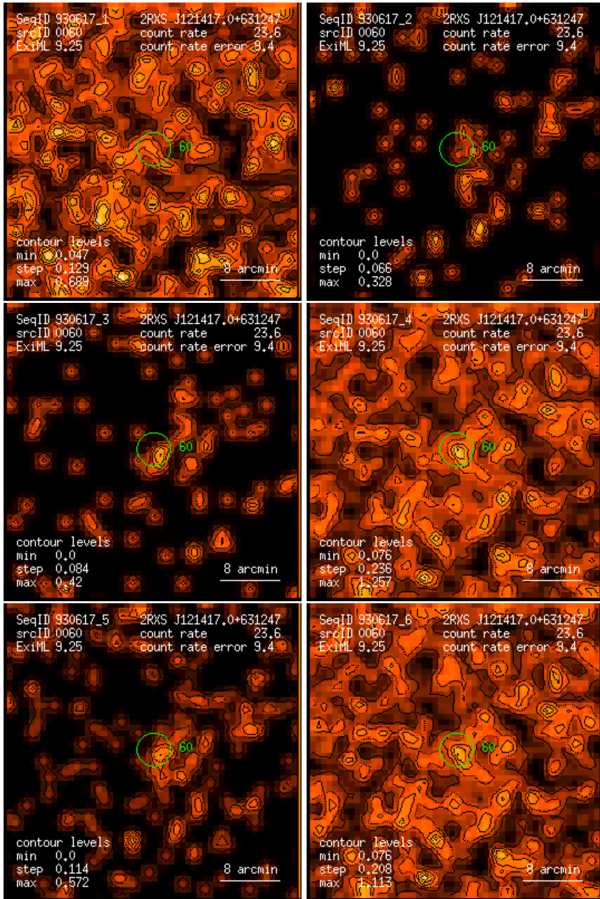
Figure 60: RASS 930617: detection 0060: band rate images, Gaussian filter: (1) PSPC channels 11 – 41, (2) 52 – 90, (3) 91 – 201, (4) 11 – 235, (5) 52 – 201, (6) 11 – 201. Broad band rates in counts/ks. Band rate contour levels in counts/ks/arcmin 2 .
