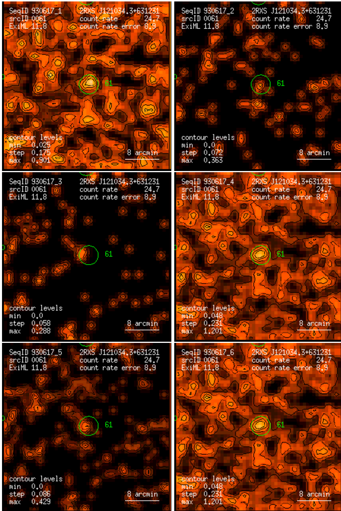
Figure 61: RASS 930617: detection 0061: band rate images, Gaussian filter: (1) PSPC channels 11 – 41, (2) 52 – 90, (3) 91 – 201, (4) 11 – 235, (5) 52 – 201, (6) 11 – 201. Broad band rates in counts/ks. Band rate contour levels in counts/ks/arcmin 2 .
