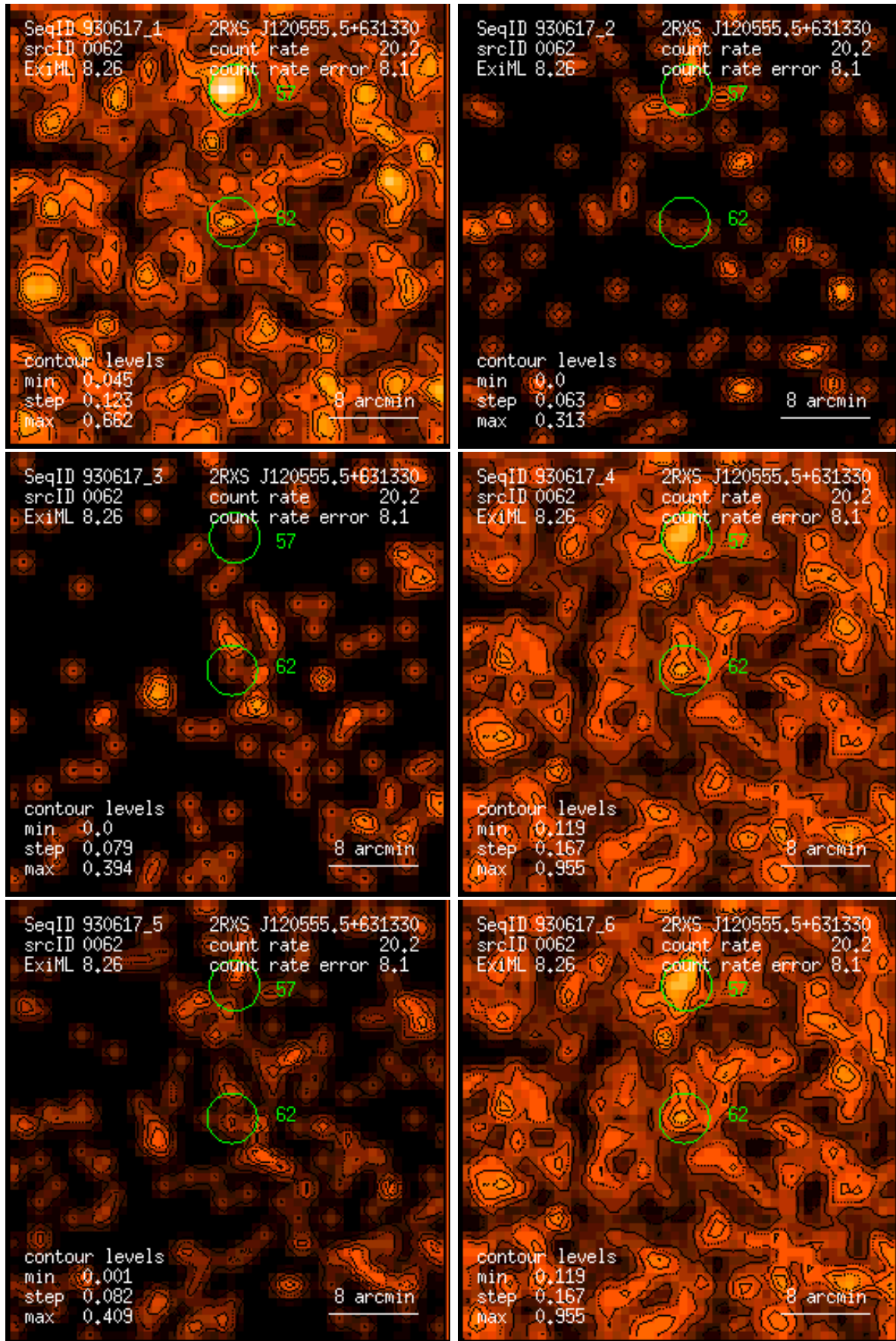
Figure 62: RASS 930617: detection 0062: band rate images, Gaussian filter: (1) PSPC channels 11 – 41, (2) 52 – 90, (3) 91 – 201, (4) 11 – 235, (5) 52 – 201, (6) 11 – 201. Broad band rates in counts/ks. Band rate contour levels in counts/ks/arcmin 2 .
