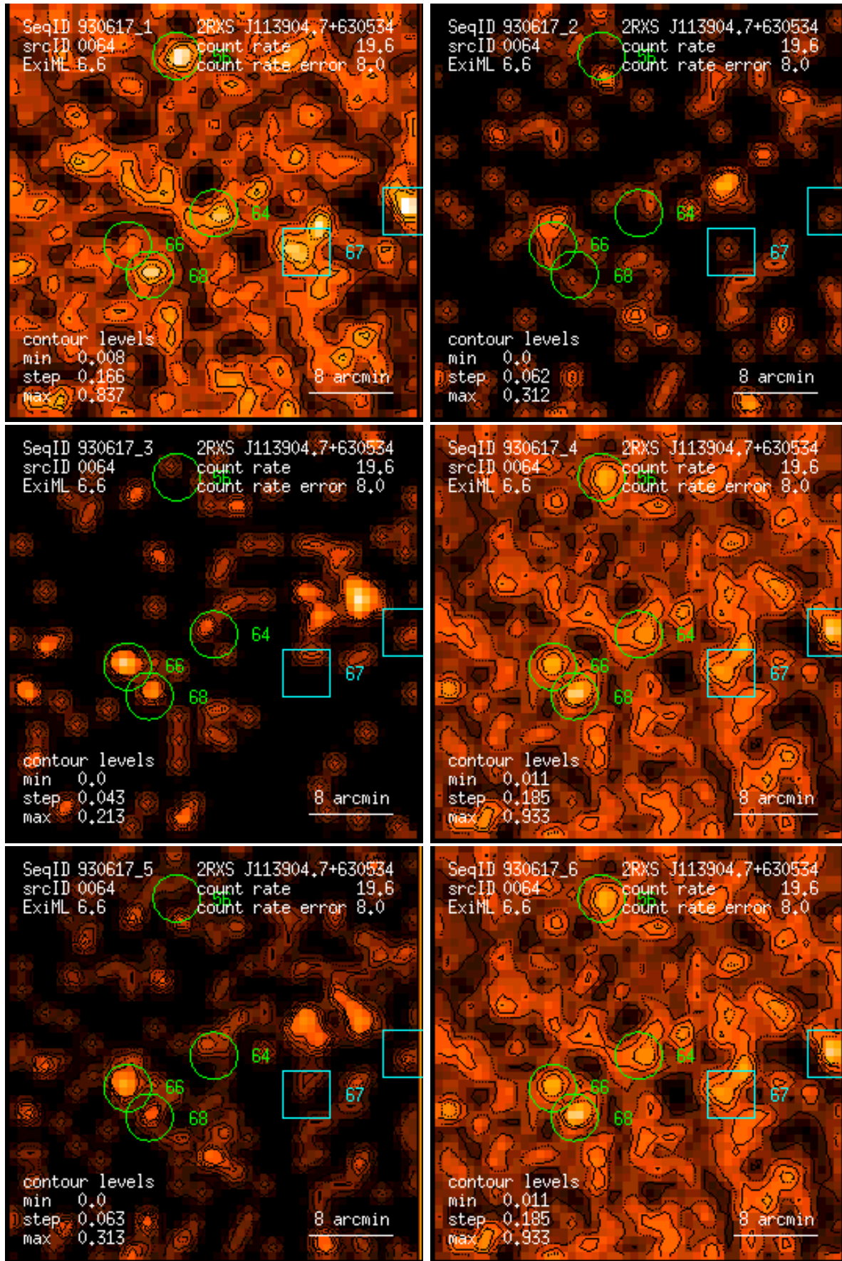
Figure 64: RASS 930617: detection 0064: band rate images, Gaussian filter: (1) PSPC channels 11 – 41, (2) 52 – 90, (3) 91 – 201, (4) 11 – 235, (5) 52 – 201, (6) 11 – 201. Broad band rates in counts/ks. Band rate contour levels in counts/ks/arcmin 2 .
