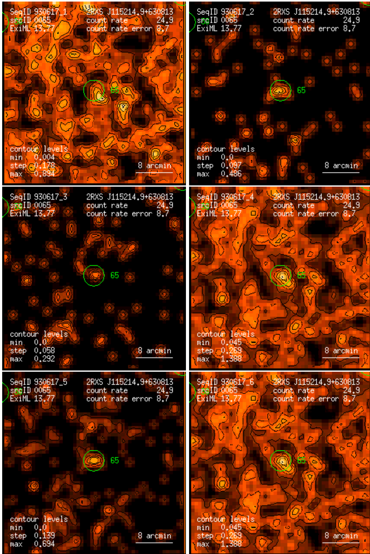
Figure 65: RASS 930617: detection 0065: band rate images, Gaussian filter: (1) PSPC channels 11 – 41, (2) 52 – 90, (3) 91 – 201, (4) 11 – 235, (5) 52 – 201, (6) 11 – 201. Broad band rates in counts/ks. Band rate contour levels in counts/ks/arcmin 2 .
