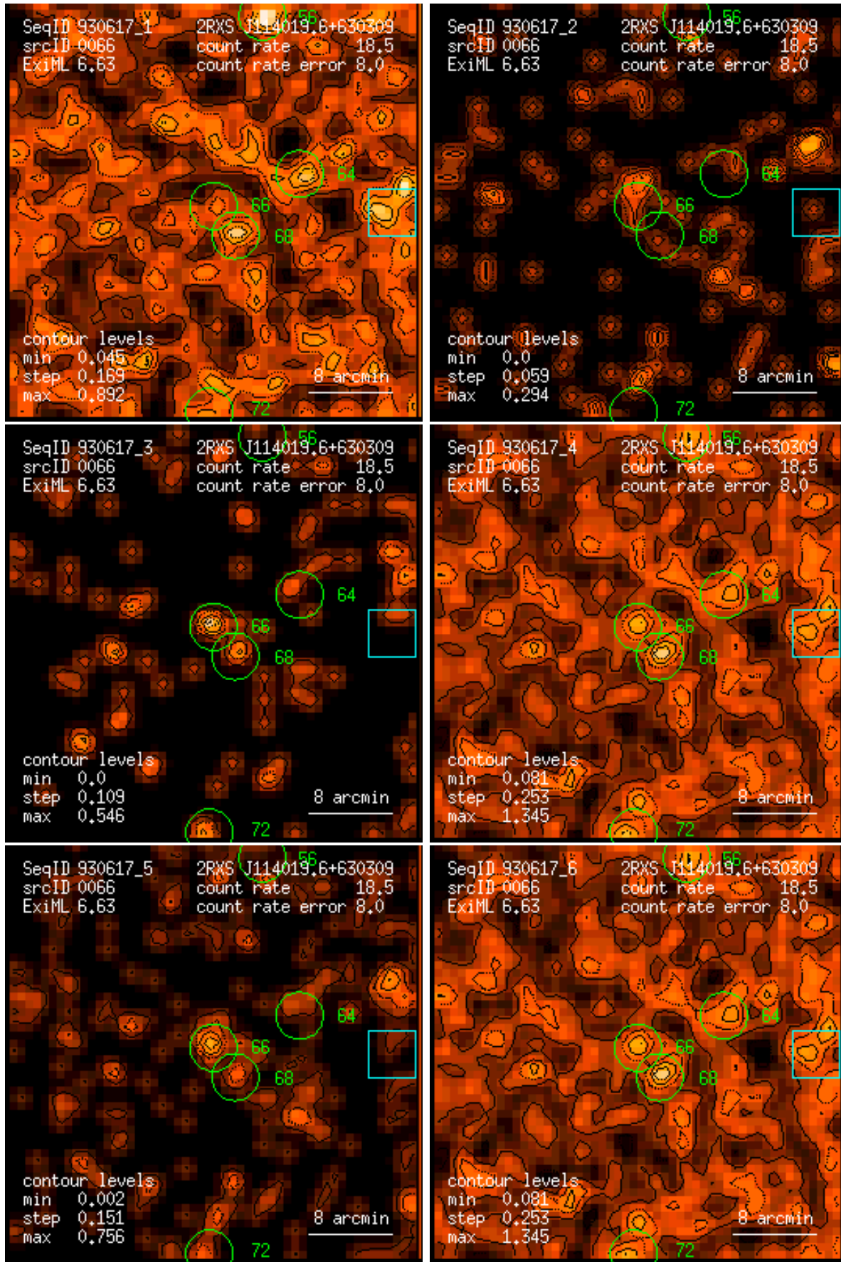
Figure 66: RASS 930617: detection 0066: band rate images, Gaussian filter: (1) PSPC channels 11 – 41, (2) 52 – 90, (3) 91 – 201, (4) 11 – 235, (5) 52 – 201, (6) 11 – 201. Broad band rates in counts/ks. Band rate contour levels in counts/ks/arcmin 2 .
