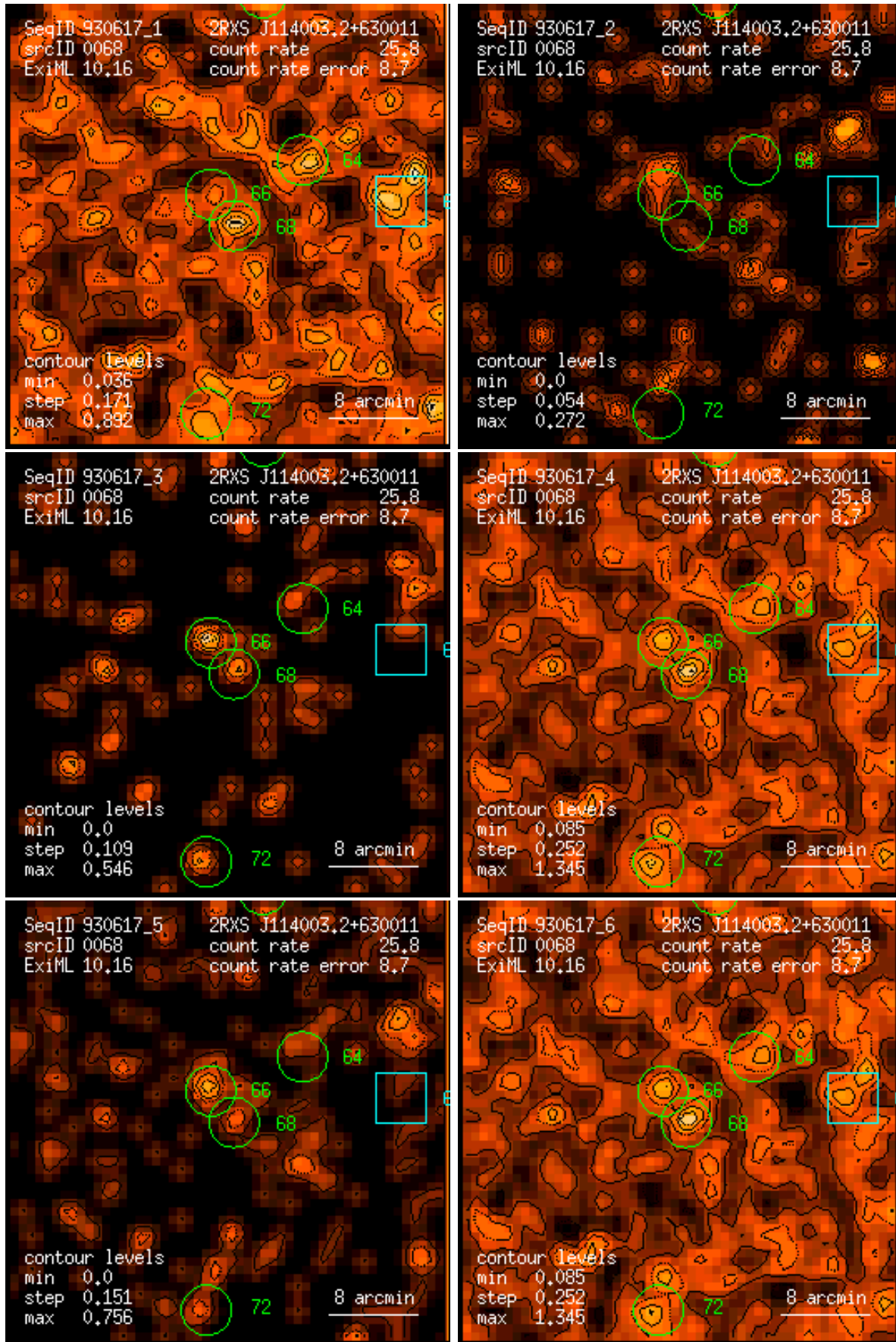
Figure 68: RASS 930617: detection 0068: band rate images, Gaussian filter: (1) PSPC channels 11 – 41, (2) 52 – 90, (3) 91 – 201, (4) 11 – 235, (5) 52 – 201, (6) 11 – 201. Broad band rates in counts/ks. Band rate contour levels in counts/ks/arcmin 2 .
