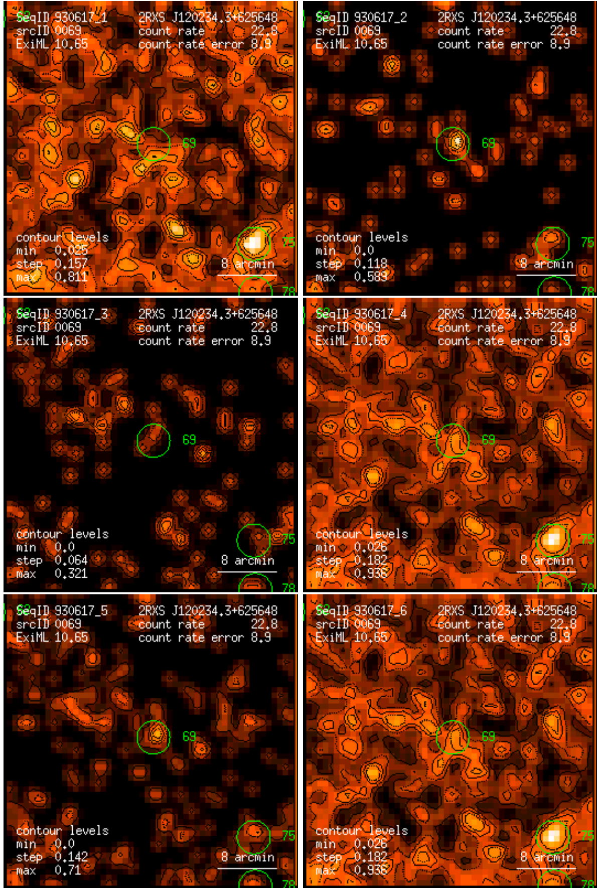
Figure 69: RASS 930617: detection 0069: band rate images, Gaussian filter: (1) PSPC channels 11 – 41, (2) 52 – 90, (3) 91 – 201, (4) 11 – 235, (5) 52 – 201, (6) 11 – 201. Broad band rates in counts/ks. Band rate contour levels in counts/ks/arcmin 2 .
