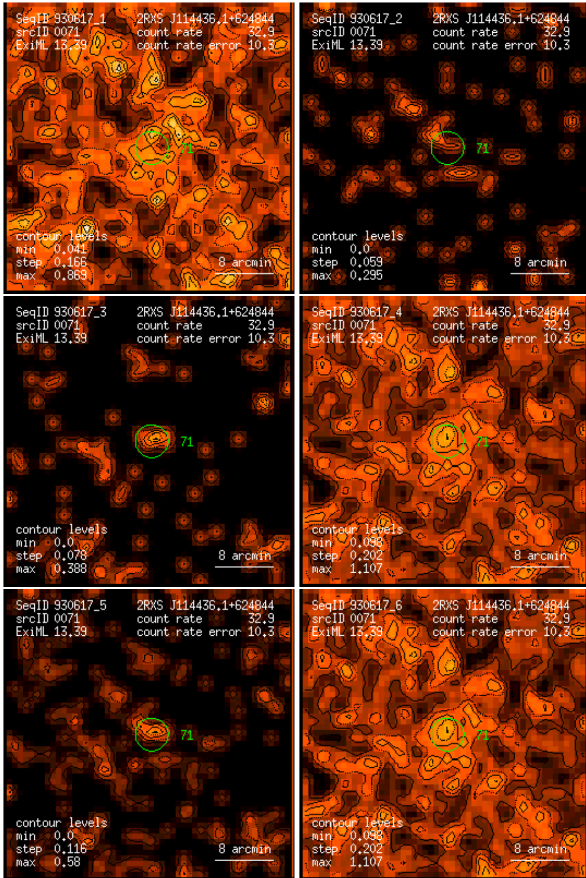
Figure 71: RASS 930617: detection 0071: band rate images, Gaussian filter: (1) PSPC channels 11 – 41, (2) 52 – 90, (3) 91 – 201, (4) 11 – 235, (5) 52 – 201, (6) 11 – 201. Broad band rates in counts/ks. Band rate contour levels in counts/ks/arcmin 2 .
