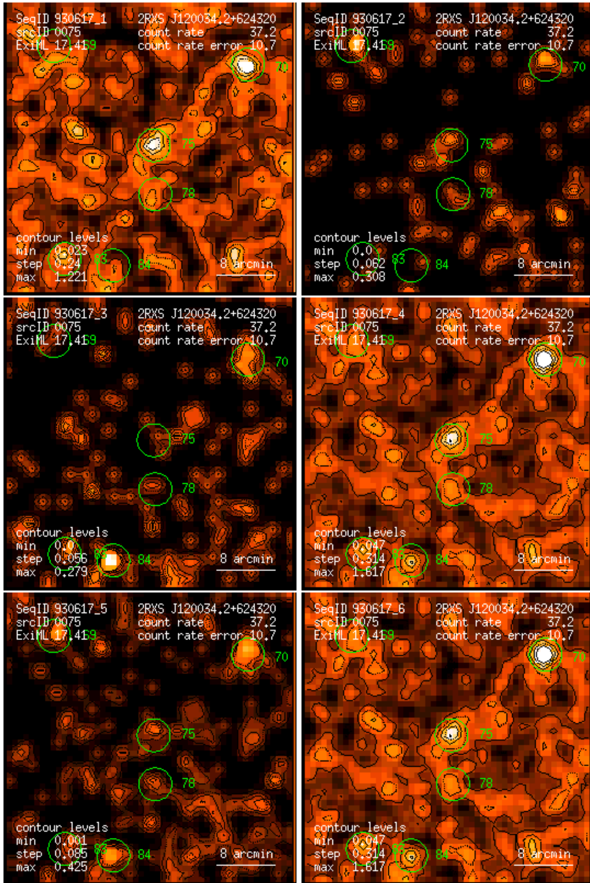
Figure 75: RASS 930617: detection 0075: band rate images, Gaussian filter: (1) PSPC channels 11 – 41, (2) 52 – 90, (3) 91 – 201, (4) 11 – 235, (5) 52 – 201, (6) 11 – 201. Broad band rates in counts/ks. Band rate contour levels in counts/ks/arcmin 2 .
