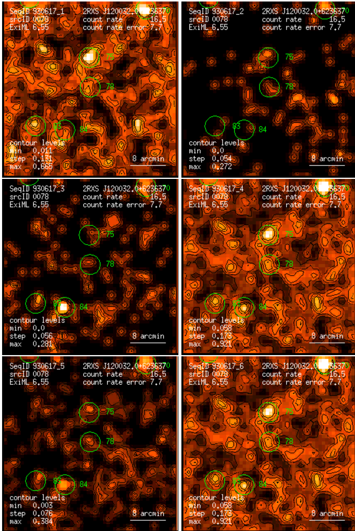
Figure 78: RASS 930617: detection 0078: band rate images, Gaussian filter: (1) PSPC channels 11 – 41, (2) 52 – 90, (3) 91 – 201, (4) 11 – 235, (5) 52 – 201, (6) 11 – 201. Broad band rates in counts/ks. Band rate contour levels in counts/ks/arcmin 2 .
