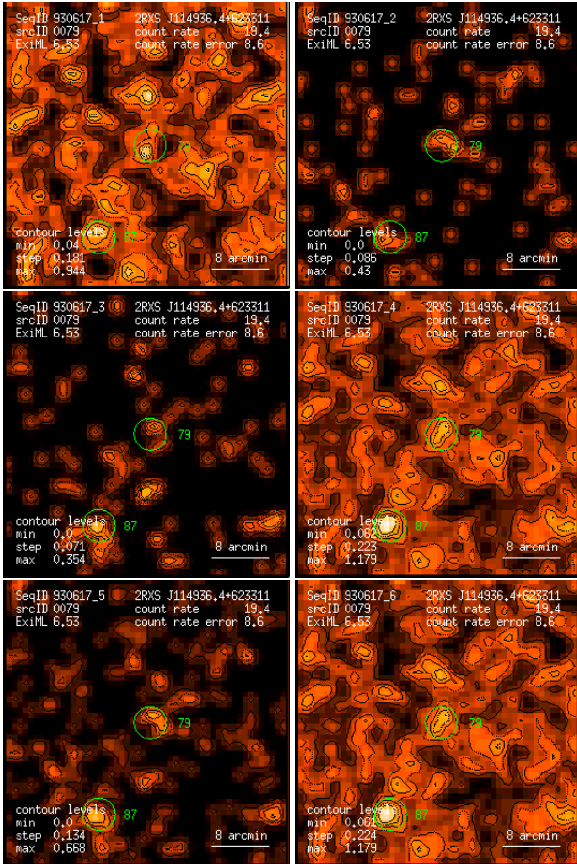
Figure 79: RASS 930617: detection 0079: band rate images, Gaussian filter: (1) PSPC channels 11 – 41, (2) 52 – 90, (3) 91 – 201, (4) 11 – 235, (5) 52 – 201, (6) 11 – 201. Broad band rates in counts/ks. Band rate contour levels in counts/ks/arcmin 2 .
