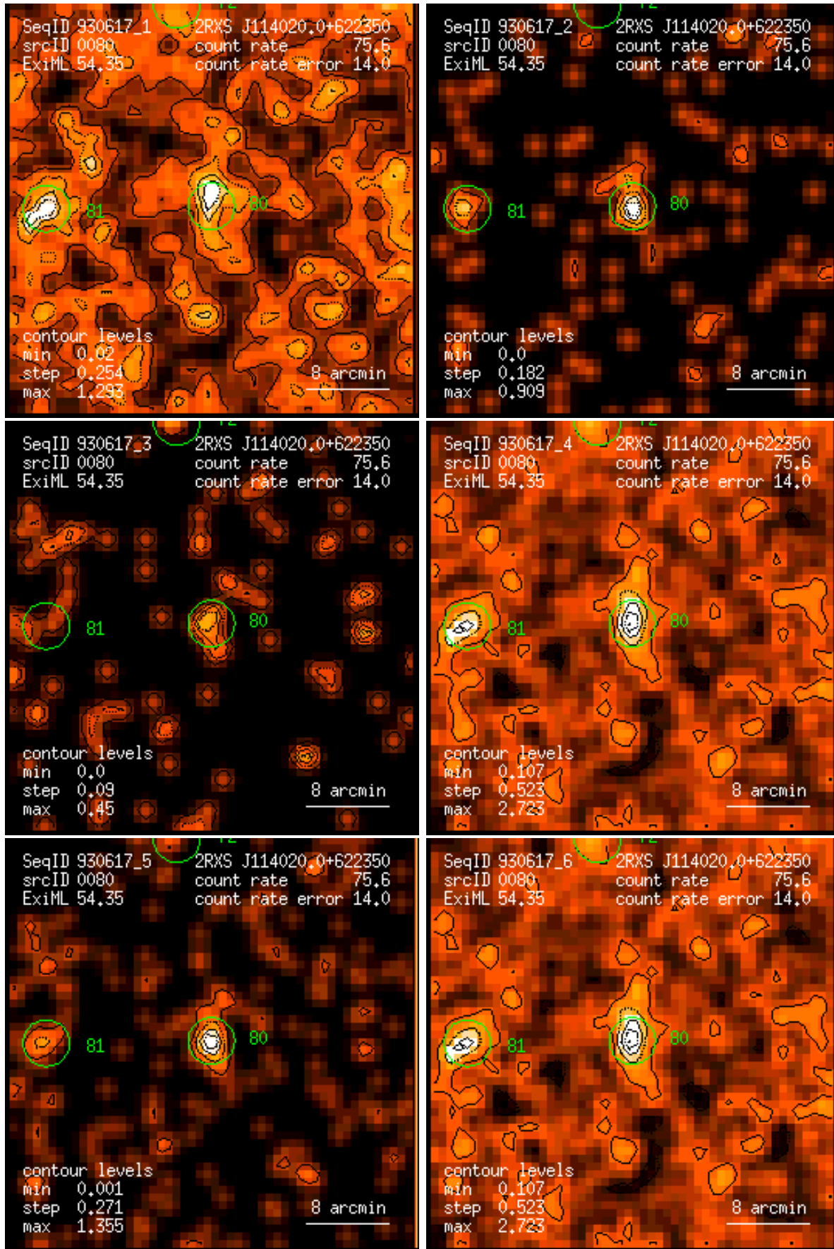
Figure 80: RASS 930617: detection 0080: band rate images, Gaussian filter: (1) PSPC channels 11 – 41, (2) 52 – 90, (3) 91 – 201, (4) 11 – 235, (5) 52 – 201, (6) 11 – 201. Broad band rates in counts/ks. Band rate contour levels in counts/ks/arcmin 2 .
