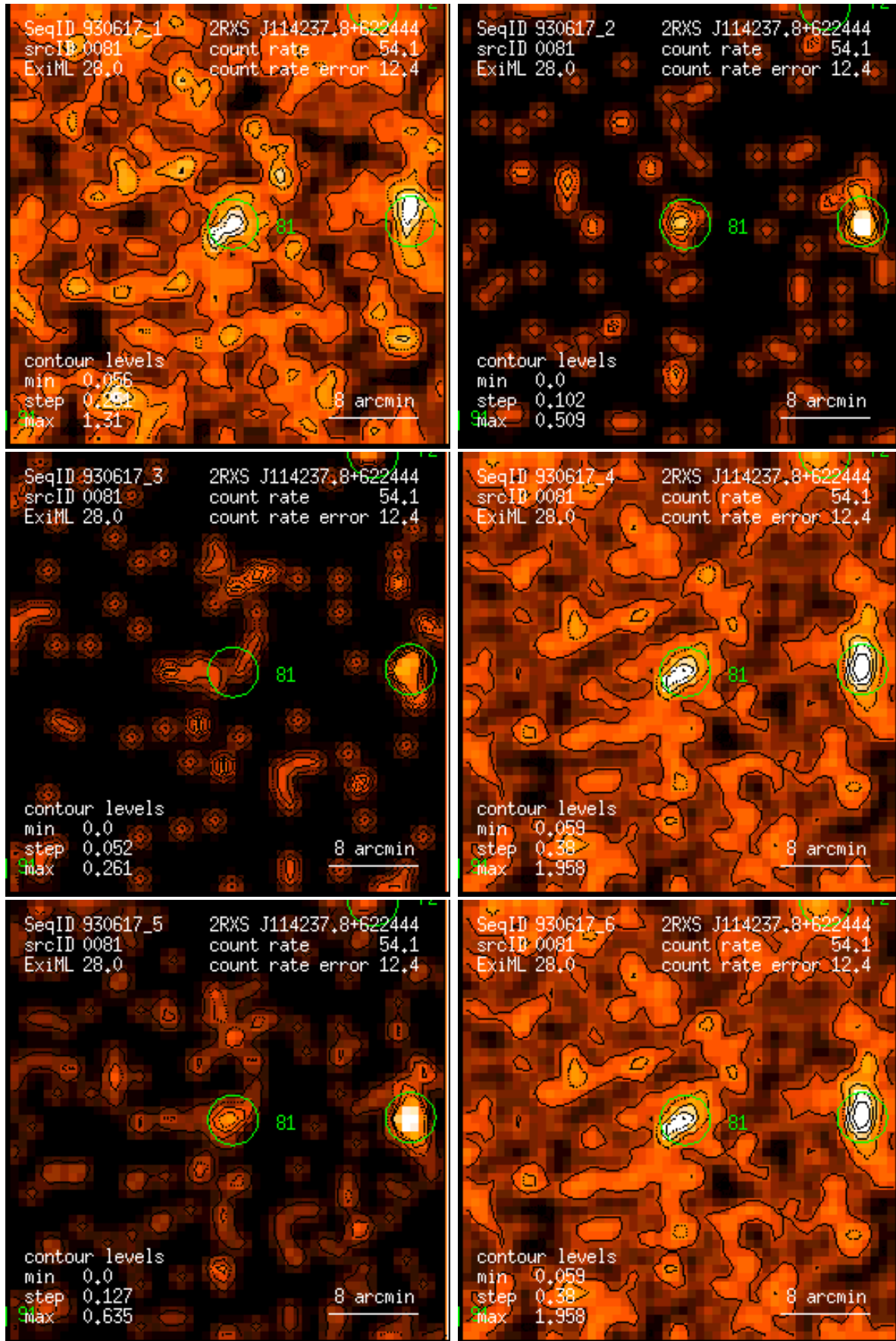
Figure 81: RASS 930617: detection 0081: band rate images, Gaussian filter: (1) PSPC channels 11 – 41, (2) 52 – 90, (3) 91 – 201, (4) 11 – 235, (5) 52 – 201, (6) 11 – 201. Broad band rates in counts/ks. Band rate contour levels in counts/ks/arcmin 2 .
