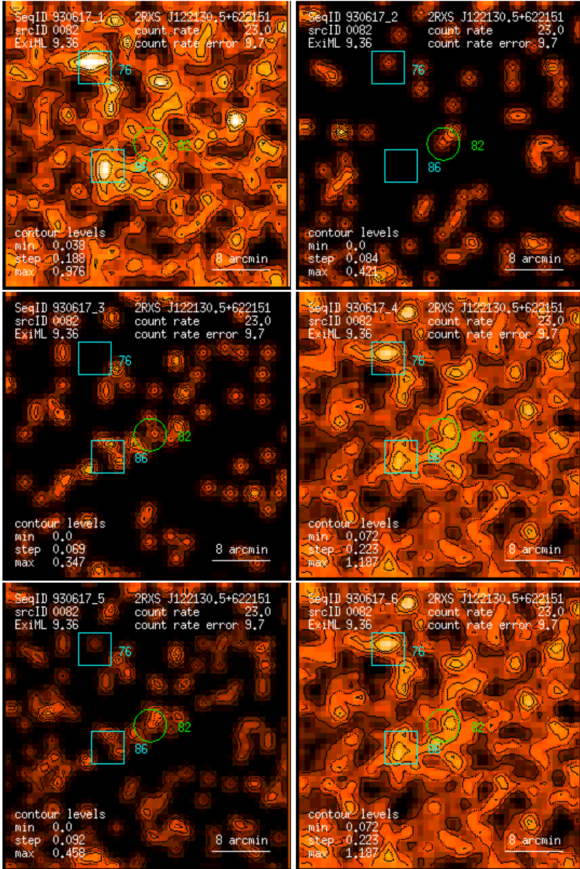
Figure 82: RASS 930617: detection 0082: band rate images, Gaussian filter: (1) PSPC channels 11 – 41, (2) 52 – 90, (3) 91 – 201, (4) 11 – 235, (5) 52 – 201, (6) 11 – 201. Broad band rates in counts/ks. Band rate contour levels in counts/ks/arcmin 2 .
