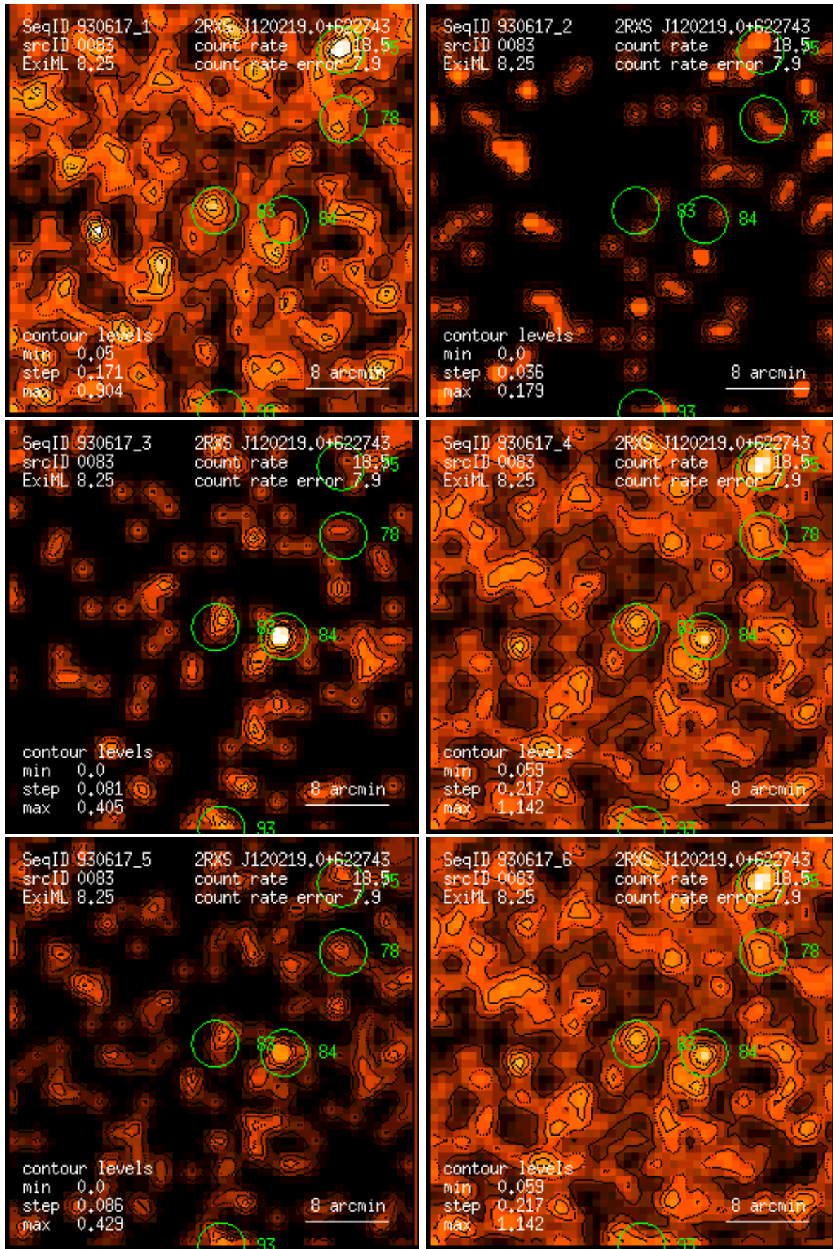
Figure 83: RASS 930617: detection 0083: band rate images, Gaussian filter: (1) PSPC channels 11 – 41, (2) 52 – 90, (3) 91 – 201, (4) 11 – 235, (5) 52 – 201, (6) 11 – 201. Broad band rates in counts/ks. Band rate contour levels in counts/ks/arcmin 2 .
