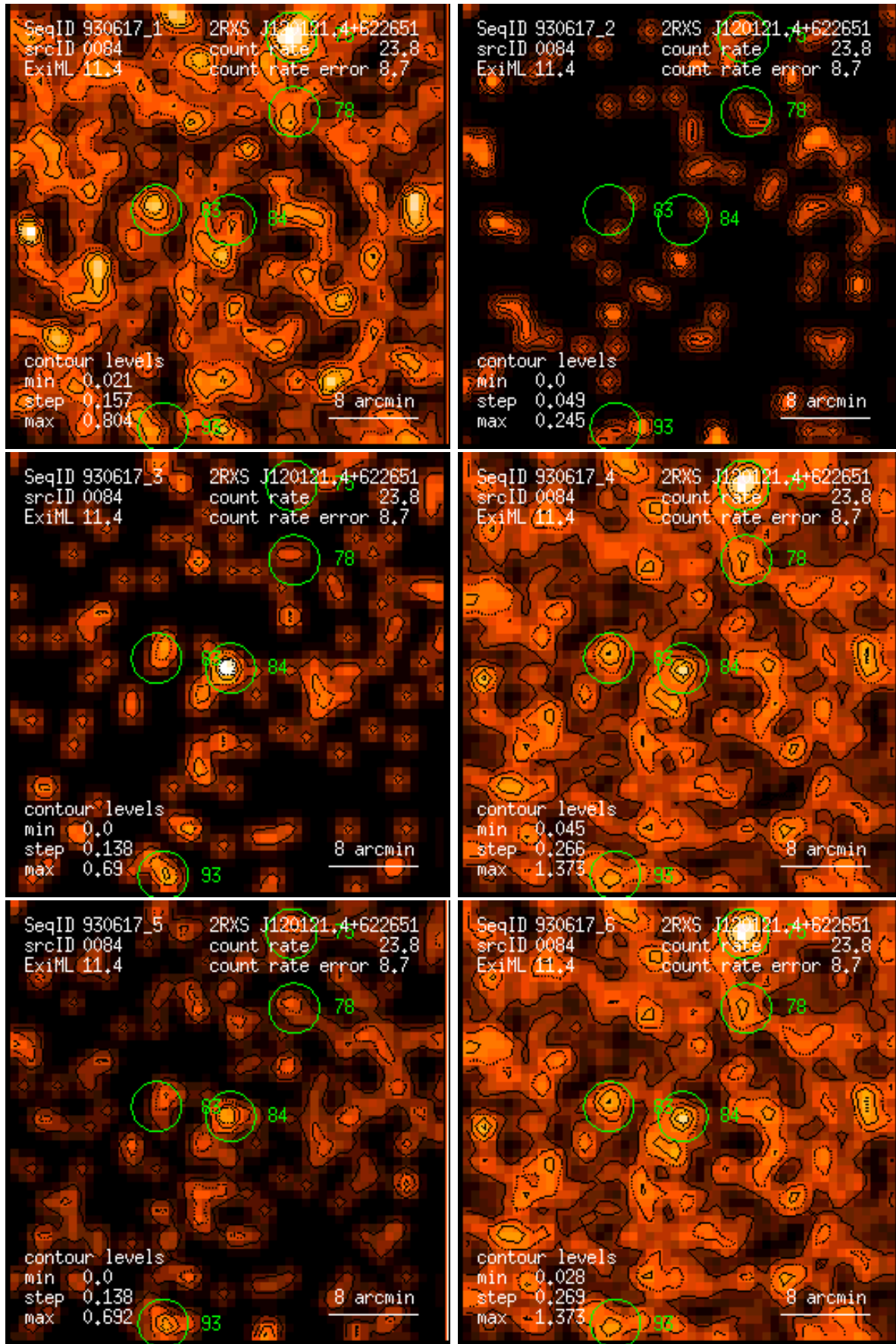
Figure 84: RASS 930617: detection 0084: band rate images, Gaussian filter: (1) PSPC channels 11 – 41, (2) 52 – 90, (3) 91 – 201, (4) 11 – 235, (5) 52 – 201, (6) 11 – 201. Broad band rates in counts/ks. Band rate contour levels in counts/ks/arcmin 2 .
