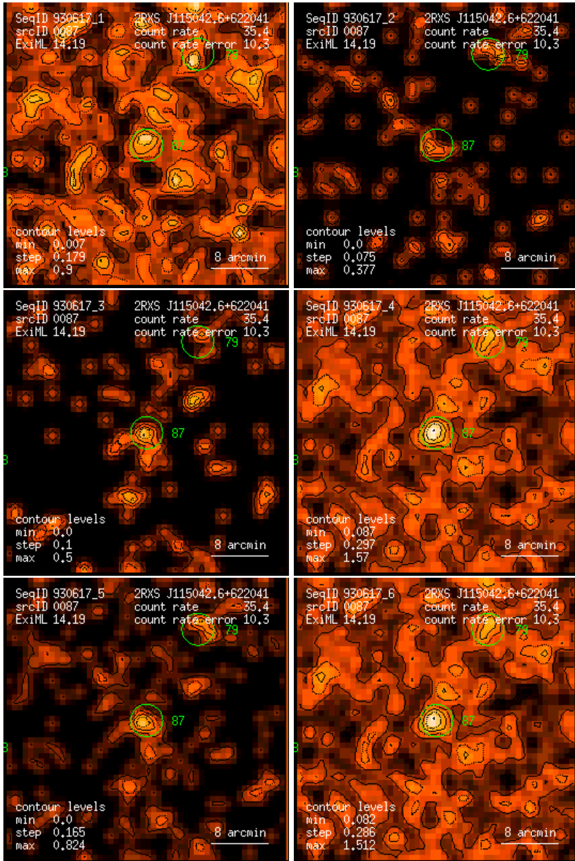
Figure 87: RASS 930617: detection 0087: band rate images, Gaussian filter: (1) PSPC channels 11 – 41, (2) 52 – 90, (3) 91 – 201, (4) 11 – 235, (5) 52 – 201, (6) 11 – 201. Broad band rates in counts/ks. Band rate contour levels in counts/ks/arcmin 2 .
