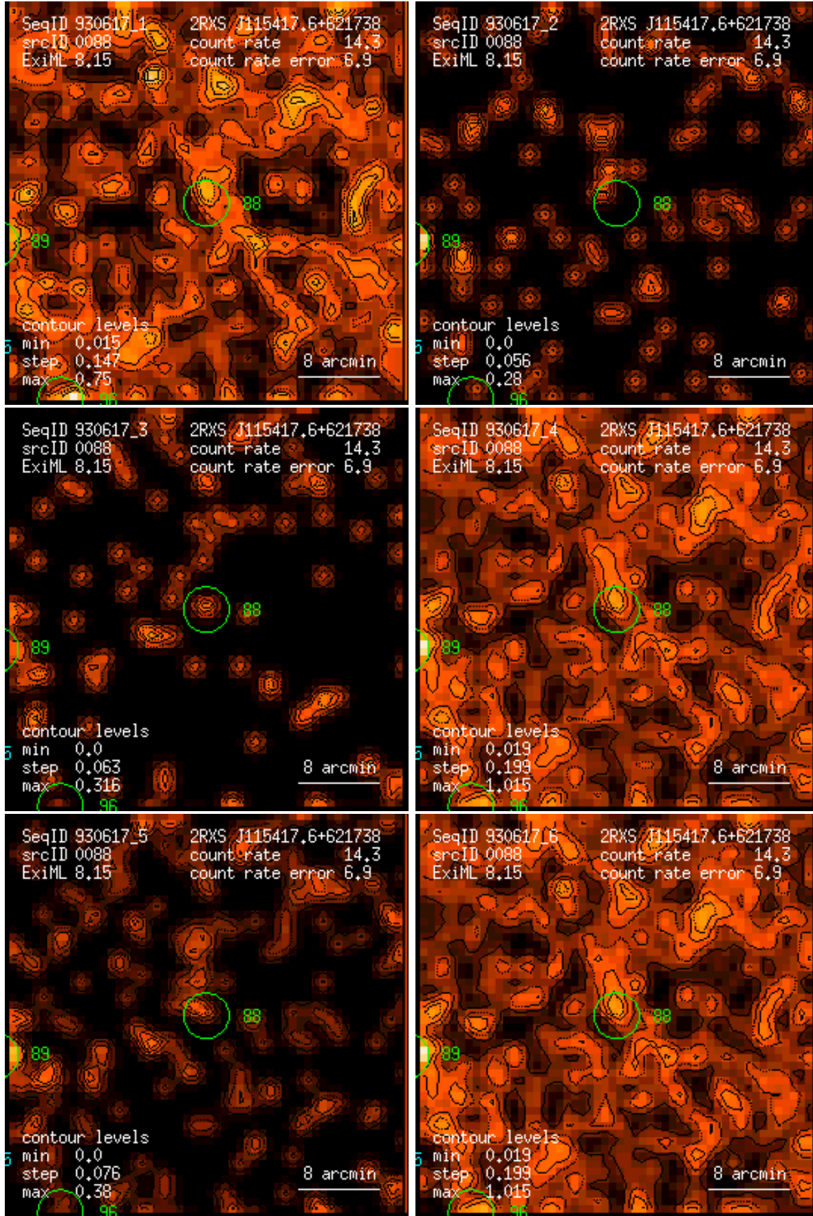
Figure 88: RASS 930617: detection 0088: band rate images, Gaussian filter: (1) PSPC channels 11 – 41, (2) 52 – 90, (3) 91 – 201, (4) 11 – 235, (5) 52 – 201, (6) 11 – 201. Broad band rates in counts/ks. Band rate contour levels in counts/ks/arcmin 2 .
