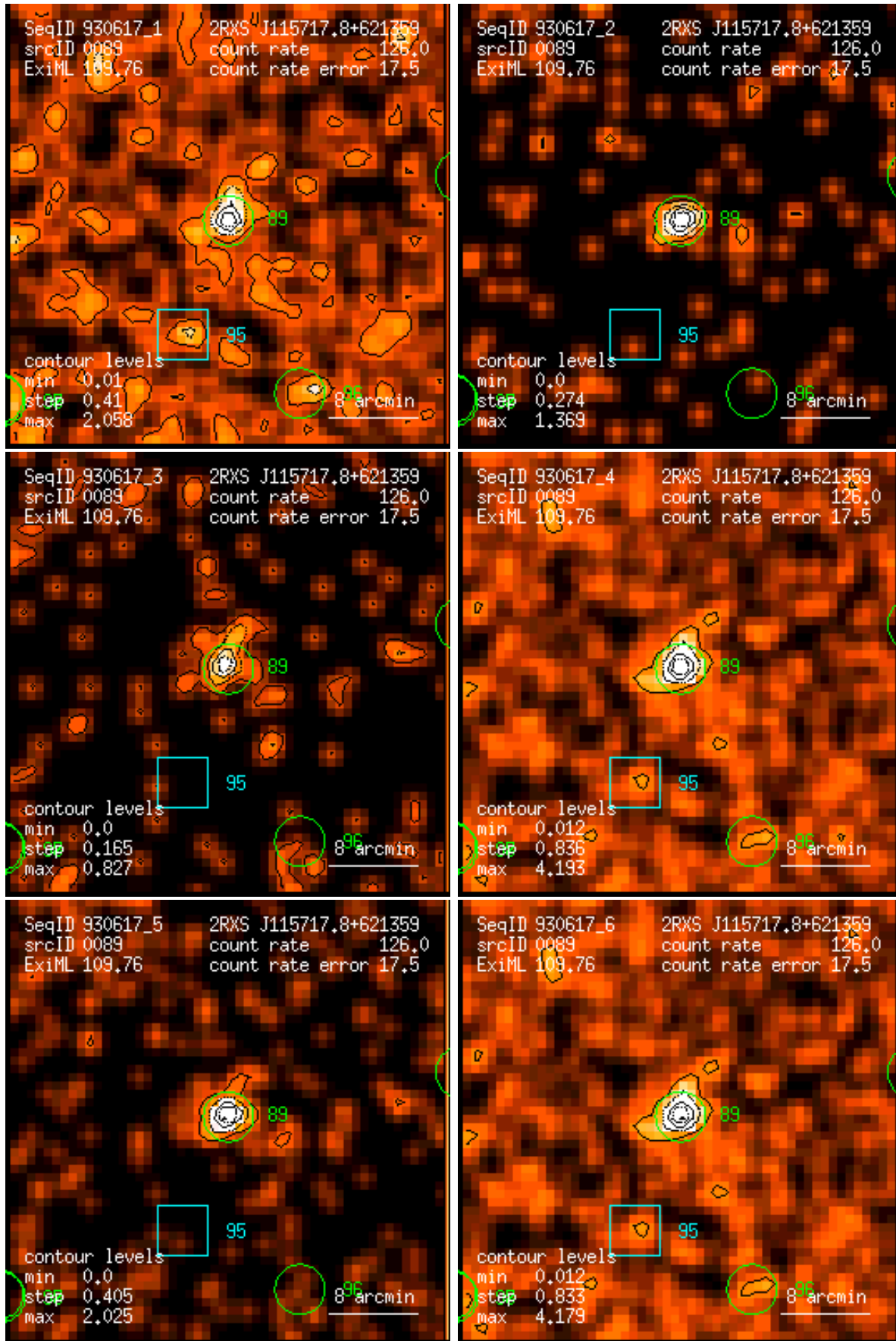
Figure 89: RASS 930617: detection 0089: band rate images, Gaussian filter: (1) PSPC channels 11 – 41, (2) 52 – 90, (3) 91 – 201, (4) 11 – 235, (5) 52 – 201, (6) 11 – 201. Broad band rates in counts/ks. Band rate contour levels in counts/ks/arcmin 2 .
