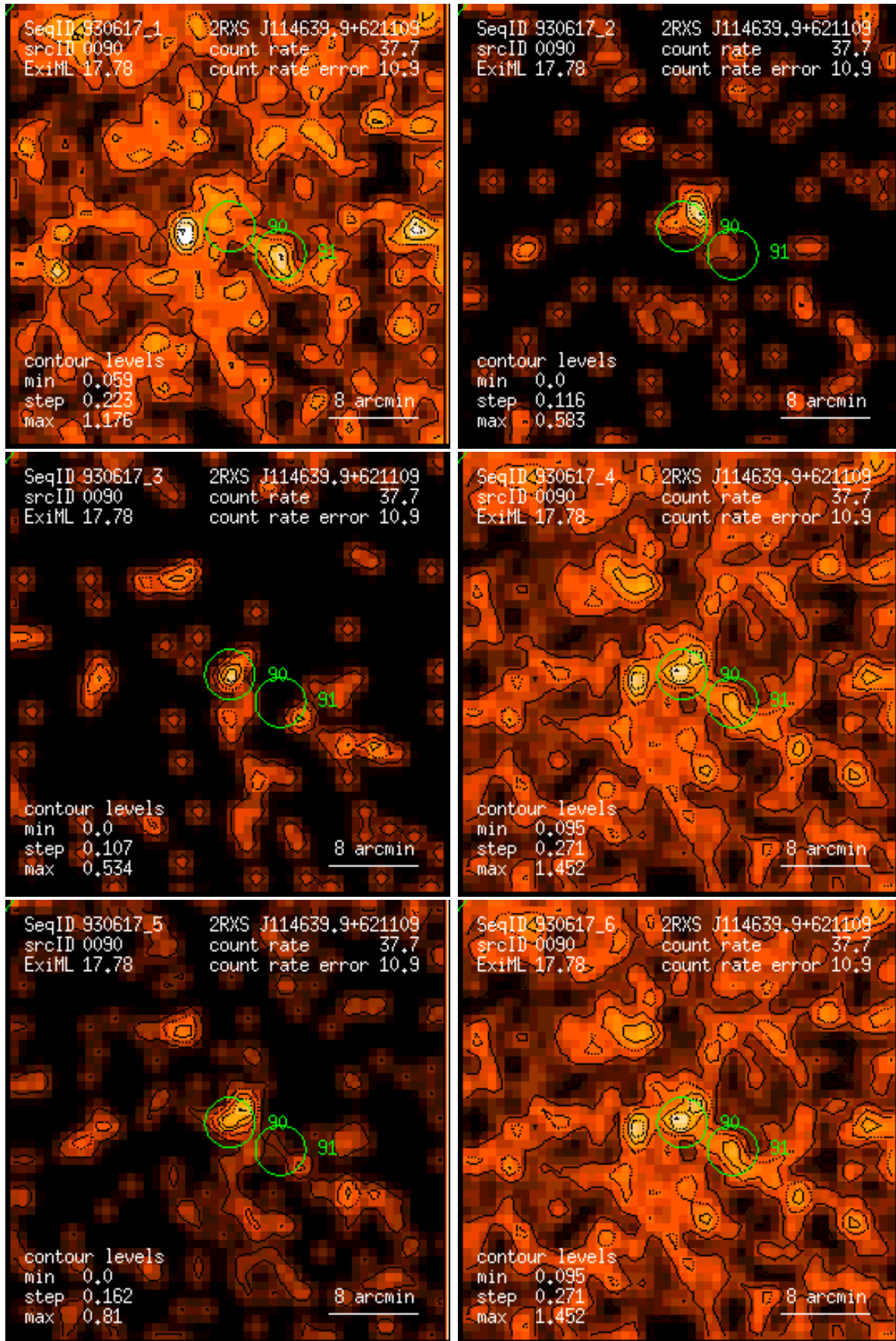
Figure 90: RASS 930617: detection 0090: band rate images, Gaussian filter: (1) PSPC channels 11 – 41, (2) 52 – 90, (3) 91 – 201, (4) 11 – 235, (5) 52 – 201, (6) 11 – 201. Broad band rates in counts/ks. Band rate contour levels in counts/ks/arcmin 2 .
