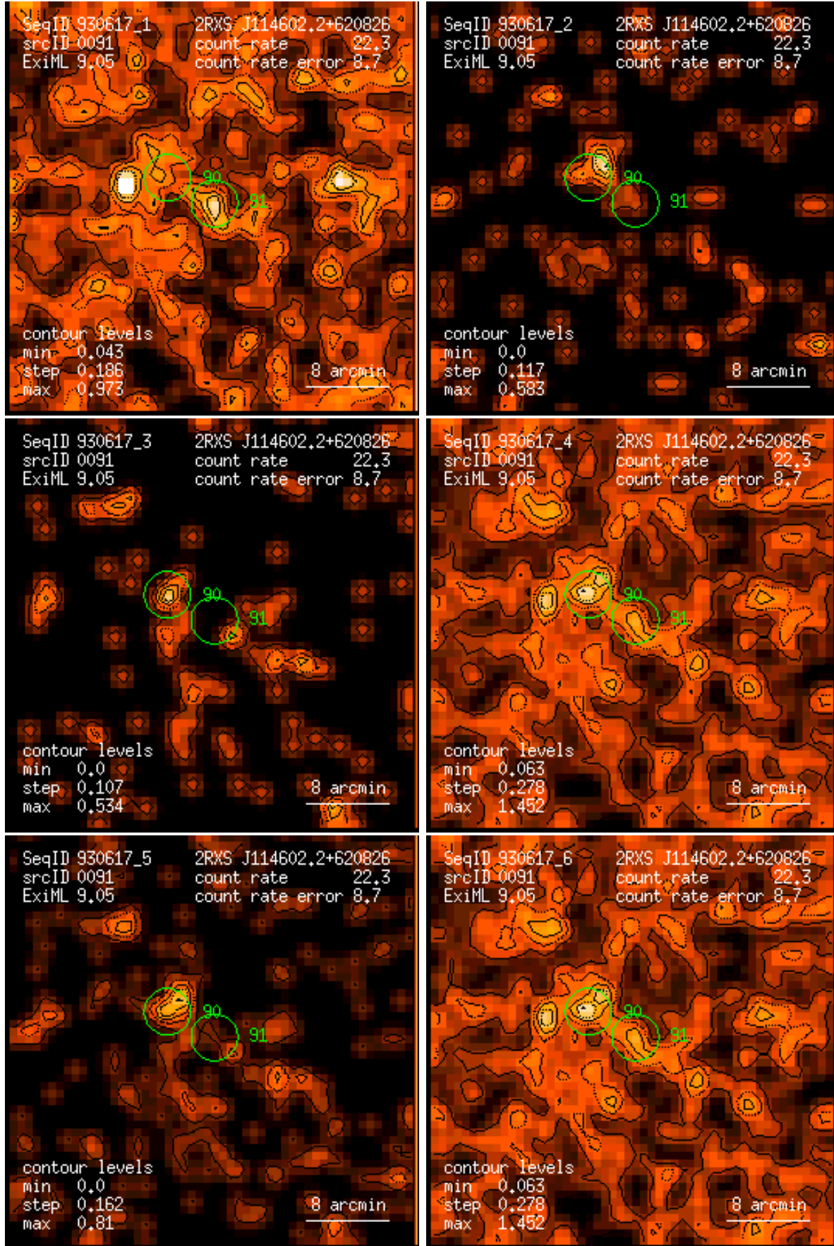
Figure 91: RASS 930617: detection 0091: band rate images, Gaussian filter: (1) PSPC channels 11 – 41, (2) 52 – 90, (3) 91 – 201, (4) 11 – 235, (5) 52 – 201, (6) 11 – 201. Broad band rates in counts/ks. Band rate contour levels in counts/ks/arcmin 2 .
