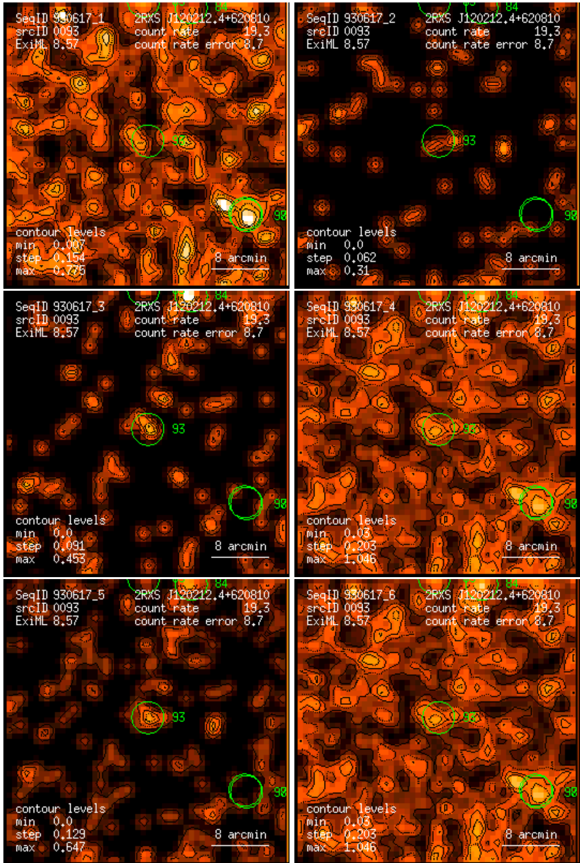
Figure 93: RASS 930617: detection 0093: band rate images, Gaussian filter: (1) PSPC channels 11 – 41, (2) 52 – 90, (3) 91 – 201, (4) 11 – 235, (5) 52 – 201, (6) 11 – 201. Broad band rates in counts/ks. Band rate contour levels in counts/ks/arcmin 2 .
