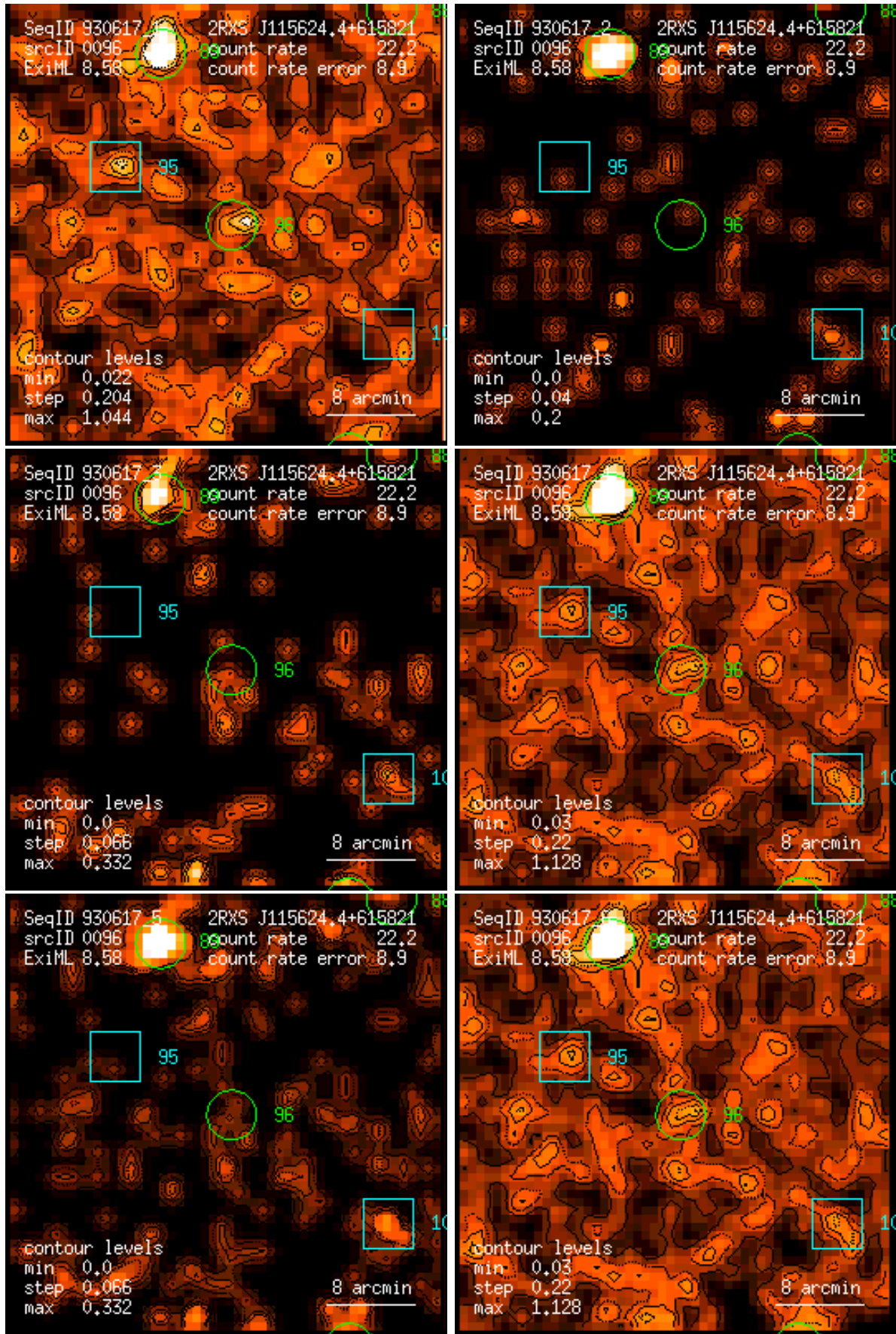
Figure 96: RASS 930617: detection 0096: band rate images, Gaussian filter: (1) PSPC channels 11 – 41, (2) 52 – 90, (3) 91 – 201, (4) 11 – 235, (5) 52 – 201, (6) 11 – 201. Broad band rates in counts/ks. Band rate contour levels in counts/ks/arcmin 2 .
