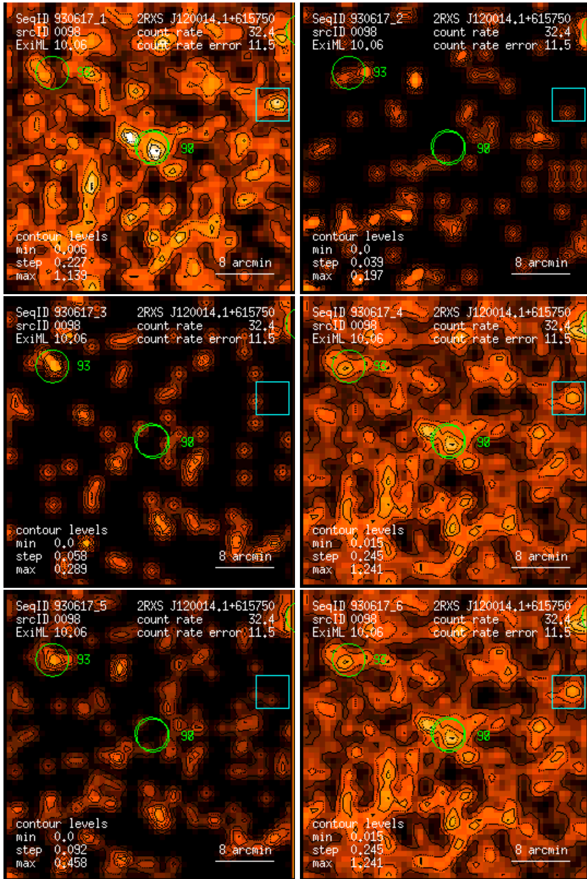
Figure 98: RASS 930617: detection 0098: band rate images, Gaussian filter: (1) PSPC channels 11 – 41, (2) 52 – 90, (3) 91 – 201, (4) 11 – 235, (5) 52 – 201, (6) 11 – 201. Broad band rates in counts/ks. Band rate contour levels in counts/ks/arcmin 2 .
