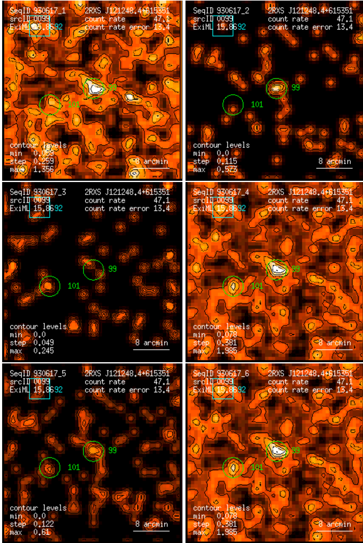
Figure 99: RASS 930617: detection 0099: band rate images, Gaussian filter: (1) PSPC channels 11 – 41, (2) 52 – 90, (3) 91 – 201, (4) 11 – 235, (5) 52 – 201, (6) 11 – 201. Broad band rates in counts/ks. Band rate contour levels in counts/ks/arcmin 2 .
