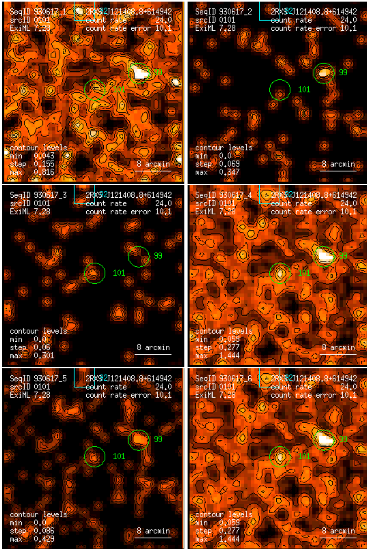
Figure 101: RASS 930617: detection 0101: band rate images, Gaussian filter: (1) PSPC channels 11 – 41, (2) 52 – 90, (3) 91 – 201, (4) 11 – 235, (5) 52 – 201, (6) 11 – 201. Broad band rates in counts/ks. Band rate contour levels in counts/ks/arcmin 2 .
