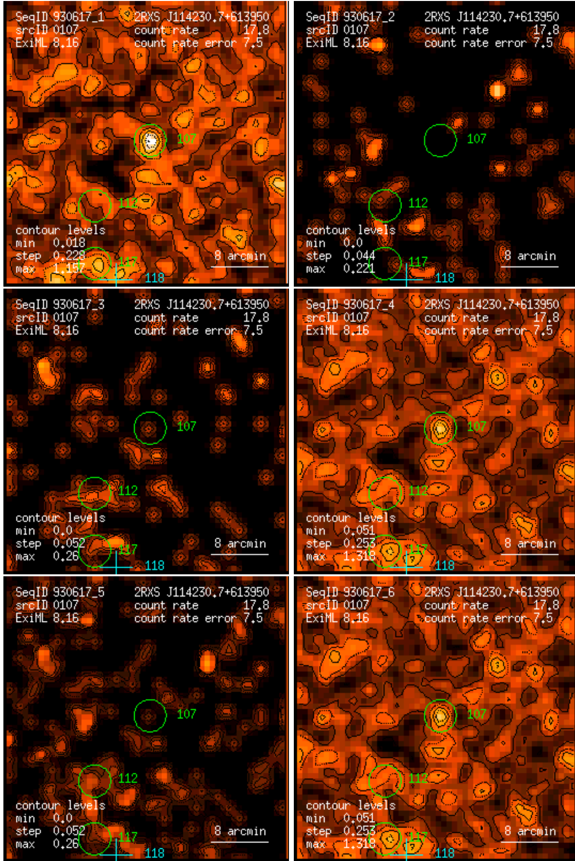
Figure 107: RASS 930617: detection 0107: band rate images, Gaussian filter: (1) PSPC channels 11 – 41, (2) 52 – 90, (3) 91 – 201, (4) 11 – 235, (5) 52 – 201, (6) 11 – 201. Broad band rates in counts/ks. Band rate contour levels in counts/ks/arcmin 2 .
