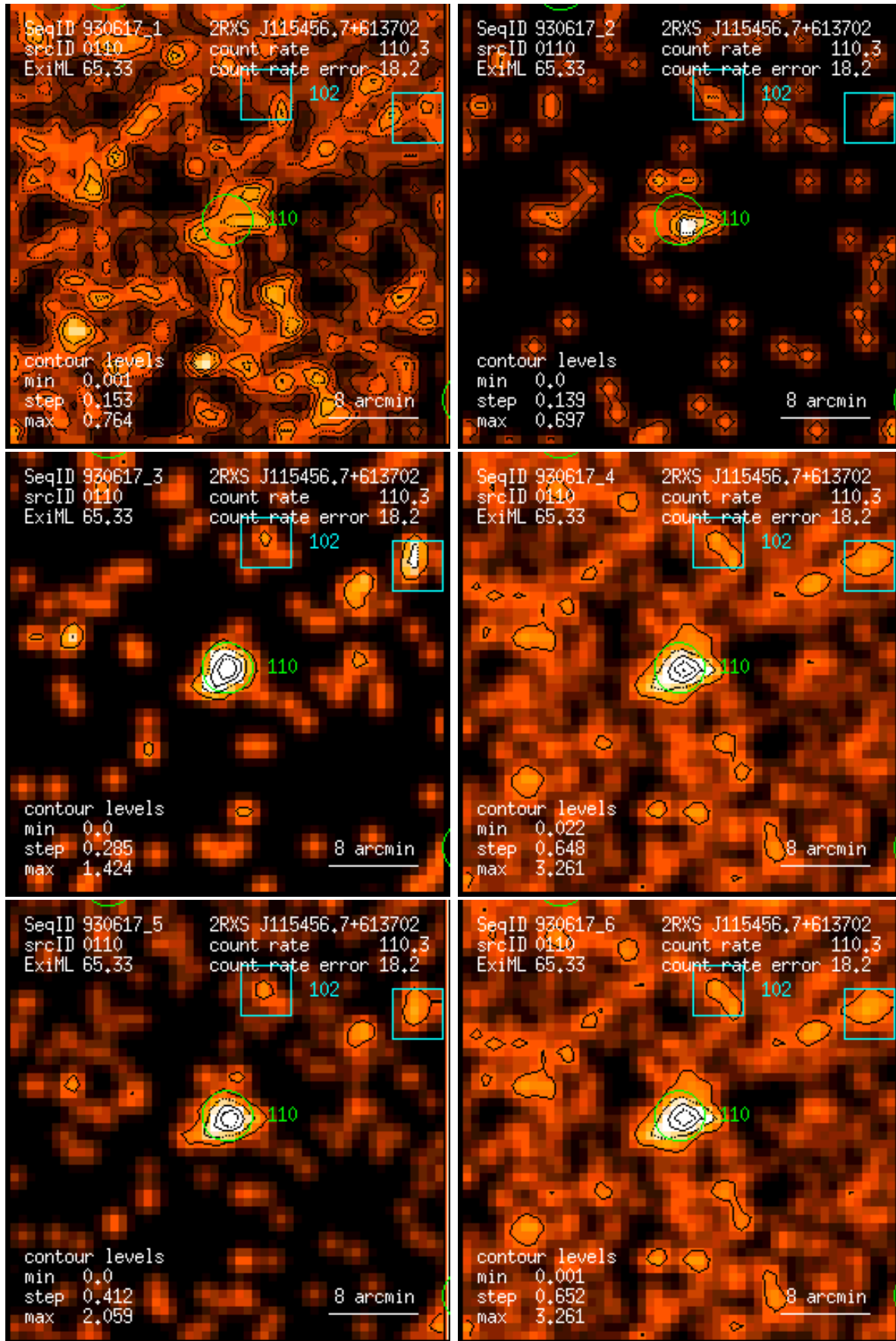
Figure 110: RASS 930617: detection 0110: band rate images, Gaussian filter: (1) PSPC channels 11 – 41, (2) 52 – 90, (3) 91 – 201, (4) 11 – 235, (5) 52 – 201, (6) 11 – 201. Broad band rates in counts/ks. Band rate contour levels in counts/ks/arcmin 2 .
