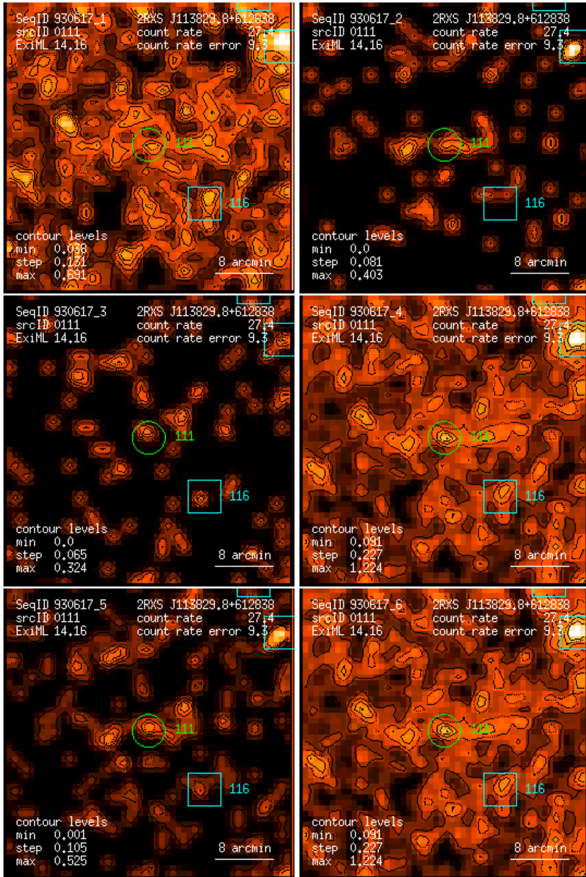
Figure 111: RASS 930617: detection 0111: band rate images, Gaussian filter: (1) PSPC channels 11 – 41, (2) 52 – 90, (3) 91 – 201, (4) 11 – 235, (5) 52 – 201, (6) 11 – 201. Broad band rates in counts/ks. Band rate contour levels in counts/ks/arcmin 2 .
