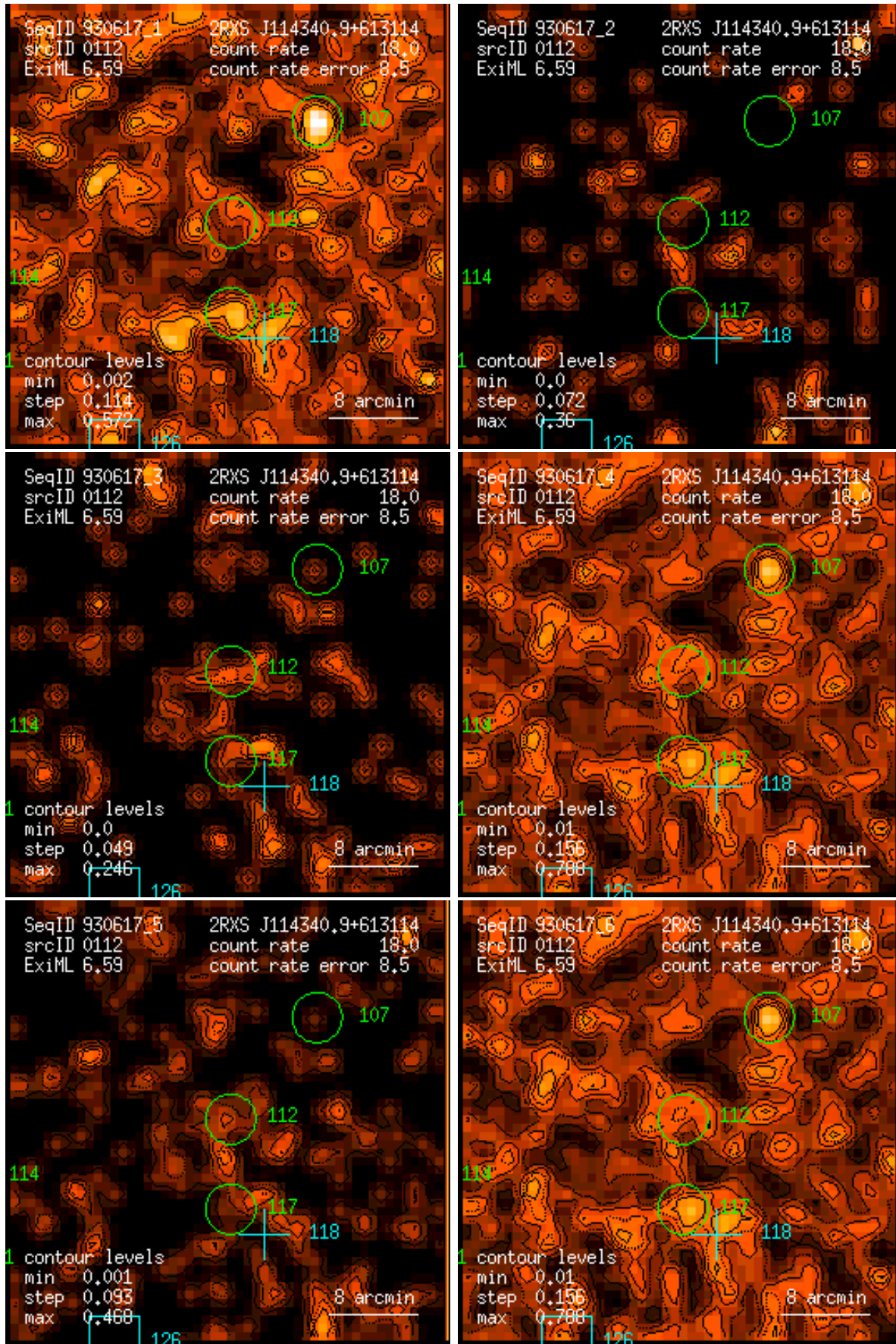
Figure 112: RASS 930617: detection 0112: band rate images, Gaussian filter: (1) PSPC channels 11 – 41, (2) 52 – 90, (3) 91 – 201, (4) 11 – 235, (5) 52 – 201, (6) 11 – 201. Broad band rates in counts/ks. Band rate contour levels in counts/ks/arcmin 2 .
