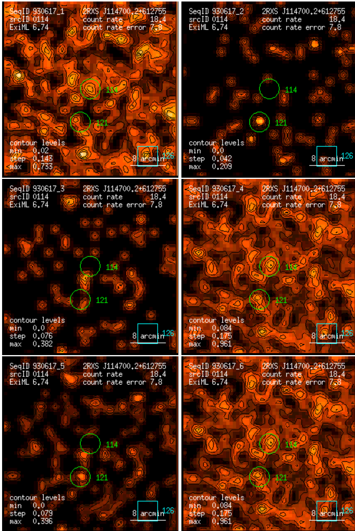
Figure 114: RASS 930617: detection 0114: band rate images, Gaussian filter: (1) PSPC channels 11 – 41, (2) 52 – 90, (3) 91 – 201, (4) 11 – 235, (5) 52 – 201, (6) 11 – 201. Broad band rates in counts/ks. Band rate contour levels in counts/ks/arcmin 2 .
