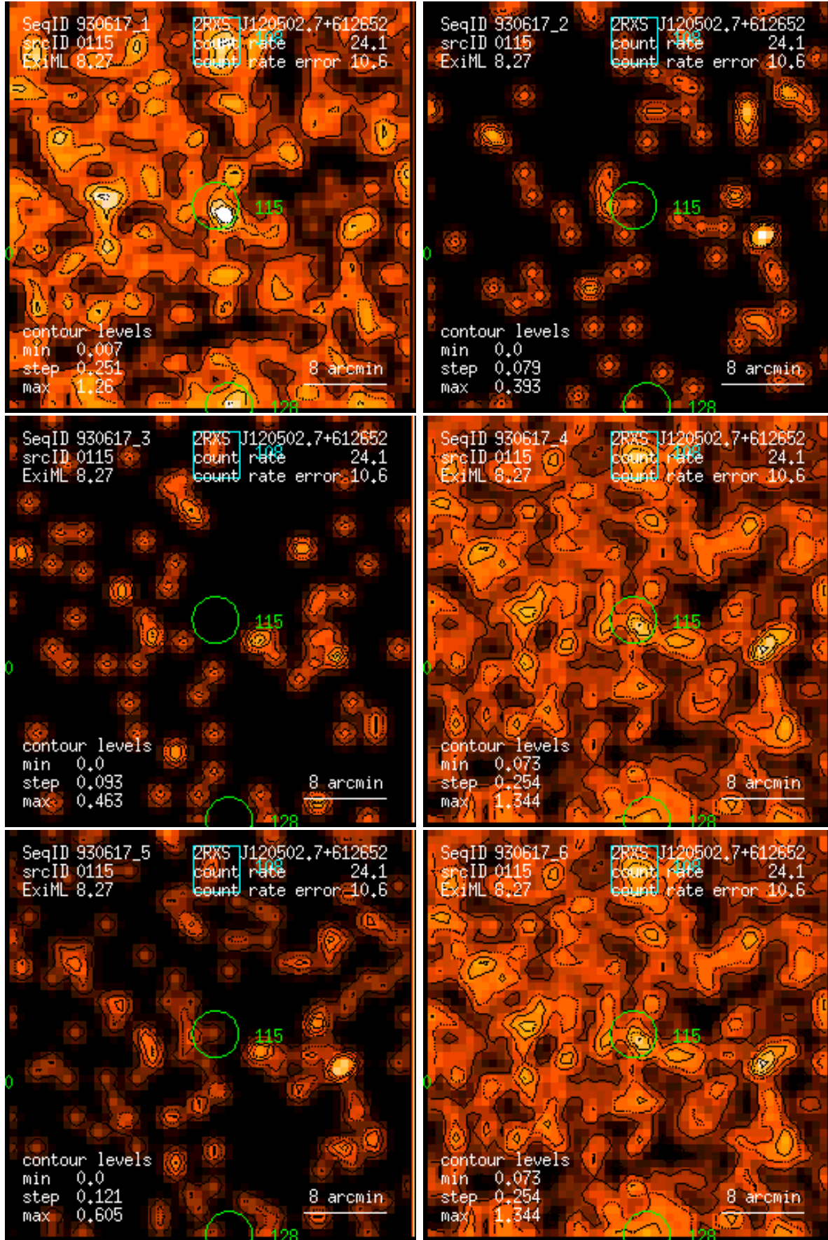
Figure 115: RASS 930617: detection 0115: band rate images, Gaussian filter: (1) PSPC channels 11 – 41, (2) 52 – 90, (3) 91 – 201, (4) 11 – 235, (5) 52 – 201, (6) 11 – 201. Broad band rates in counts/ks. Band rate contour levels in counts/ks/arcmin 2 .
