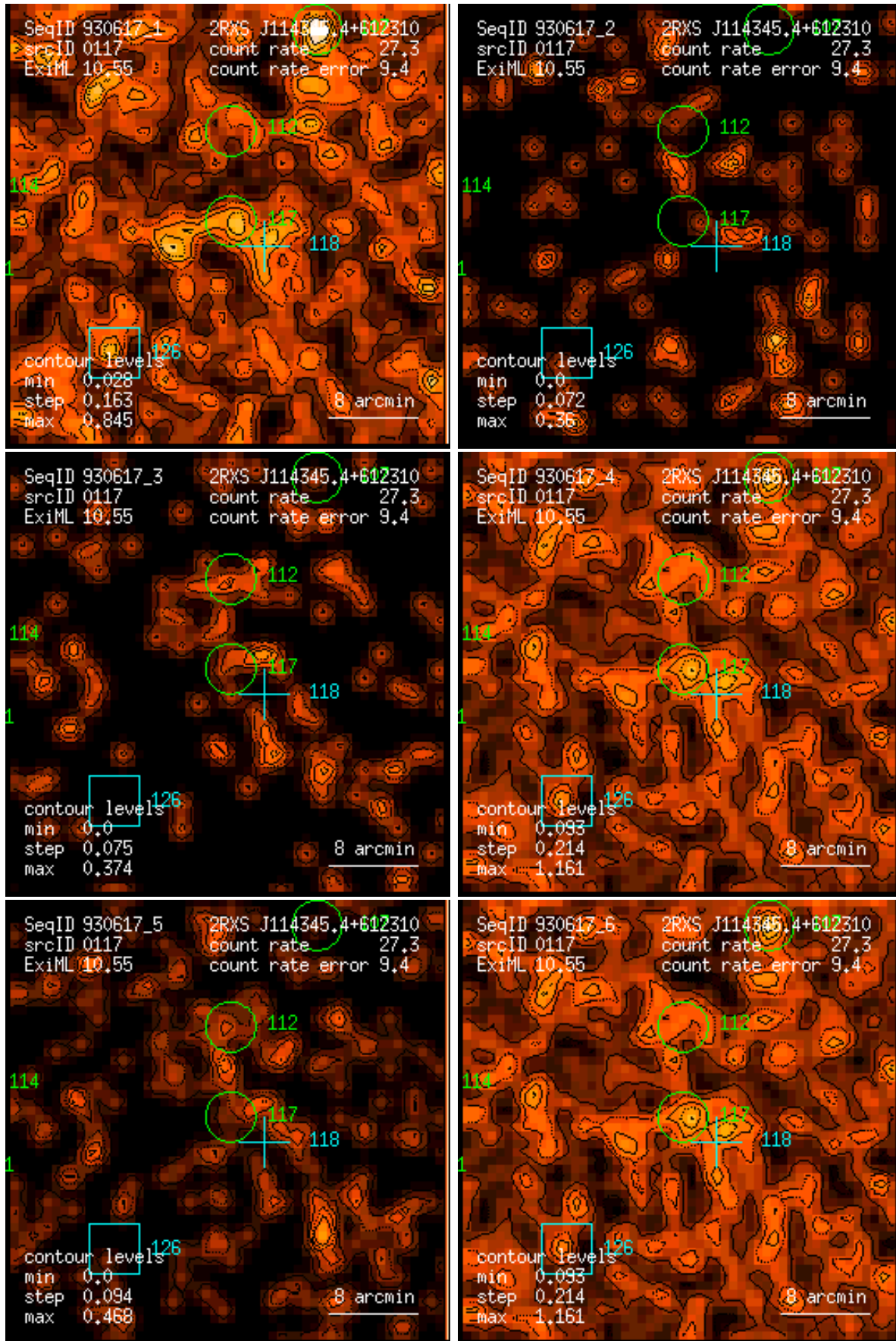
Figure 117: RASS 930617: detection 0117: band rate images, Gaussian filter: (1) PSPC channels 11 – 41, (2) 52 – 90, (3) 91 – 201, (4) 11 – 235, (5) 52 – 201, (6) 11 – 201. Broad band rates in counts/ks. Band rate contour levels in counts/ks/arcmin 2 .
