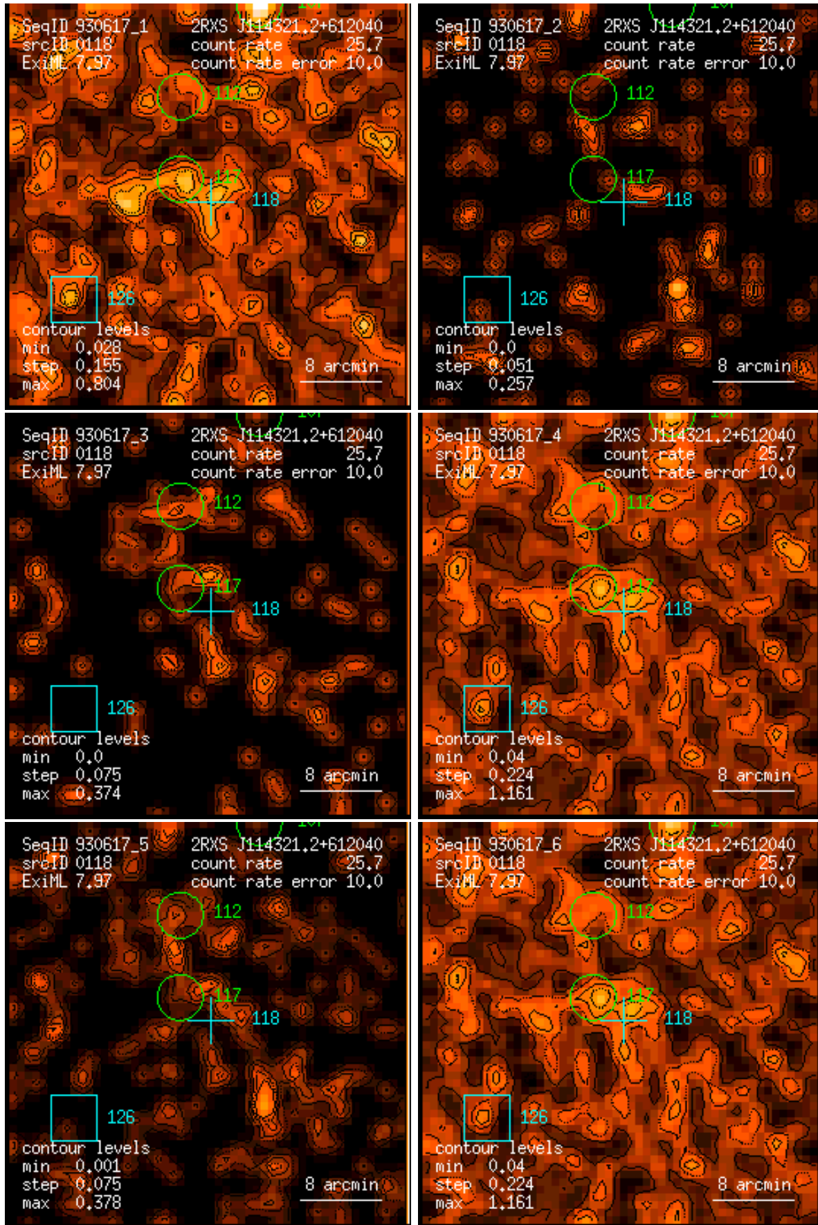
Figure 118: RASS 930617: detection 0118: band rate images, Gaussian filter: (1) PSPC channels 11 – 41, (2) 52 – 90, (3) 91 – 201, (4) 11 – 235, (5) 52 – 201, (6) 11 – 201. Broad band rates in counts/ks. Band rate contour levels in counts/ks/arcmin 2 .
